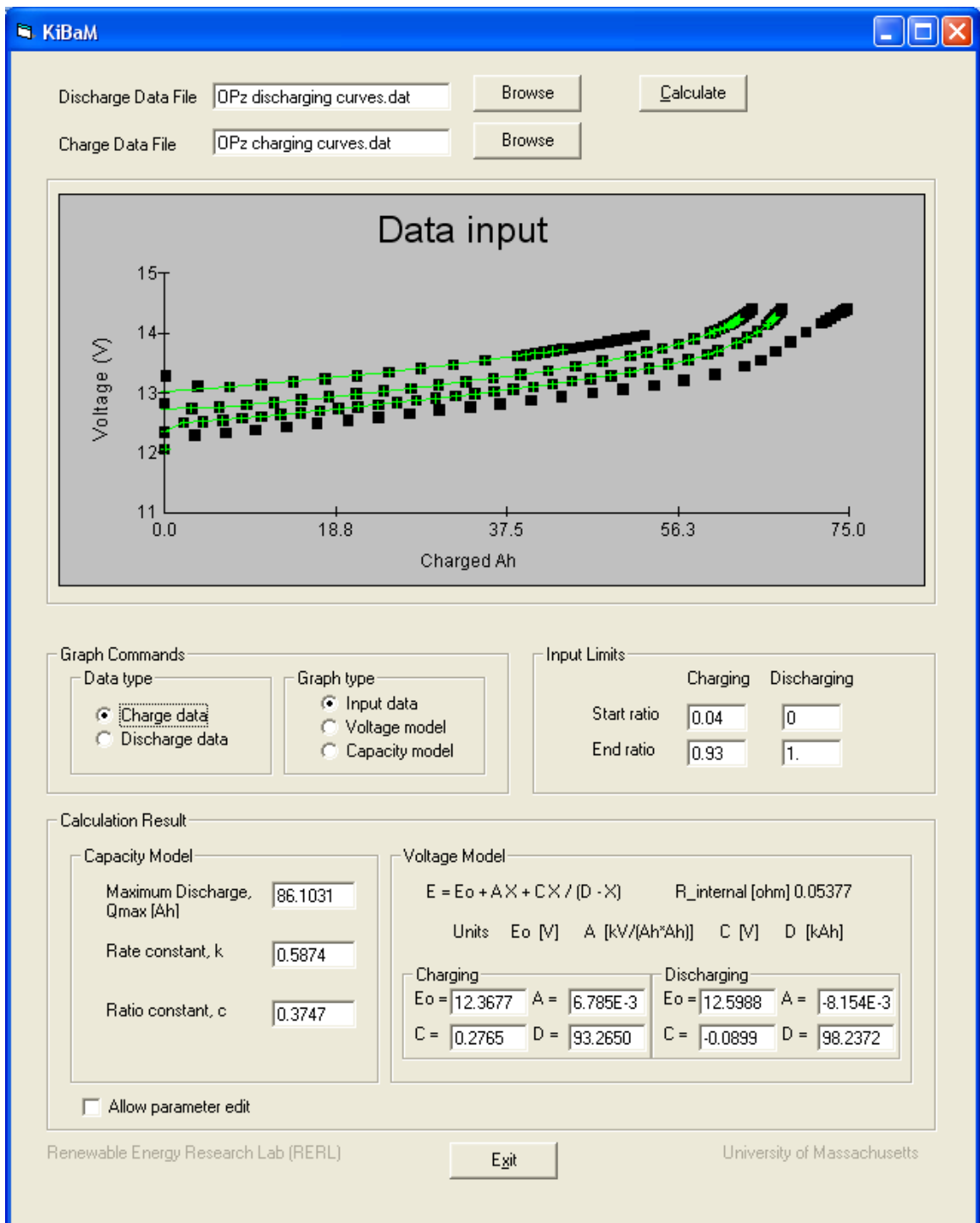
Figure 33 Voltage vs. Charge Added for OPzS Battery
