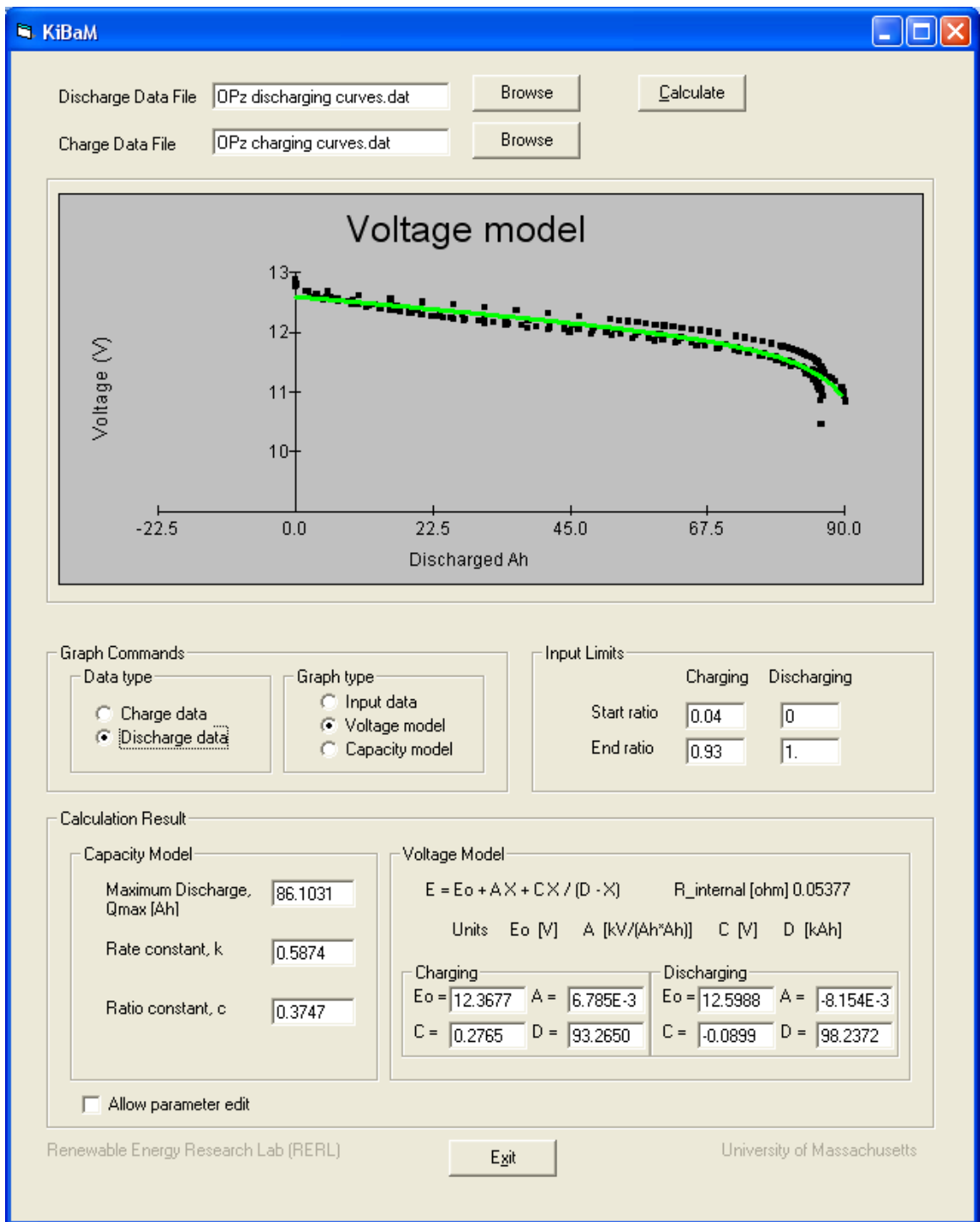
Figure 35 Determination of OPzS Discharging Voltage Constants
