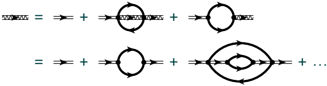
FIG. 6: Self-consistency equation for the doublon propagator (top) and some typical diagrams that make up the full propagator (bottom). Thin double-lines indicate the bare doublon propagator, the double-lines with a squiggle the full (resummed) doublon propagator, and thick single-lines the full (resummed) Fermion propagator.
