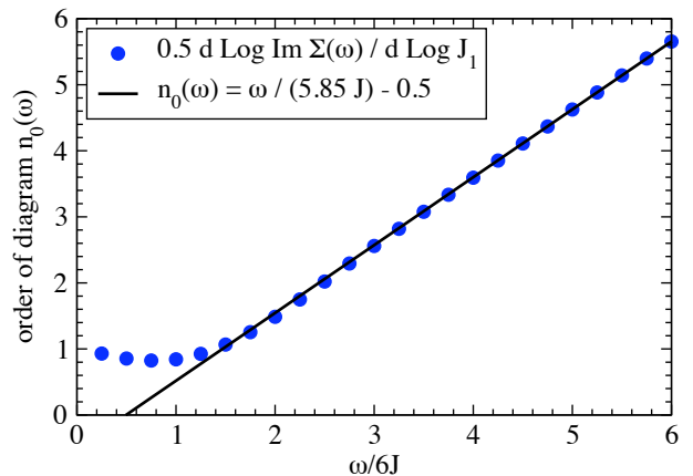
FIG. 11: Order with largest contribution to the Fermion self-energy n_0(\omega) as a function of the frequency \omega . The solid line represents the best linear fit for the high frequency data.
