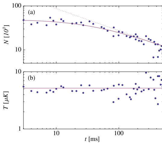
FIG. 1 (color online). Time dependence of the atom number (a) and temperature (b) for U = \eta k_B T , with T = 5.2(4) \mu\text{K} , \eta = 7.4 , and (uncorrected) L_3 = 1.2(2)_{\text{stat}} \times 10^{-21} \text{cm}^6 \text{s}^{-1} . The dotted line shows the long time t^{-1/2} dependence of the number of atoms.
