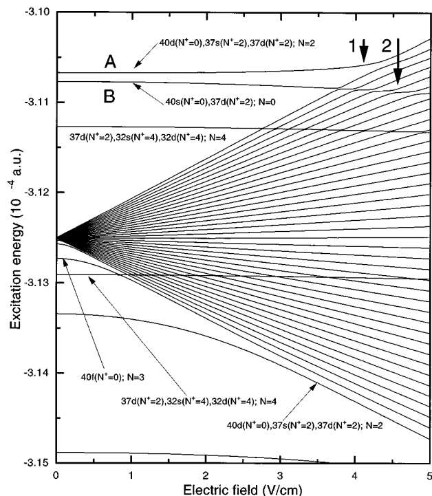
FIG. 4. Calculated Stark map in the vicinity of n=40 ( N^+=0 ) showing the energies of a number of penetrating orbitals l=0-2 ( N^+=0-4 ) and non-penetrating orbitals l \geq 3 ( N^+=0 ) as a function of the existing dc electric field.
