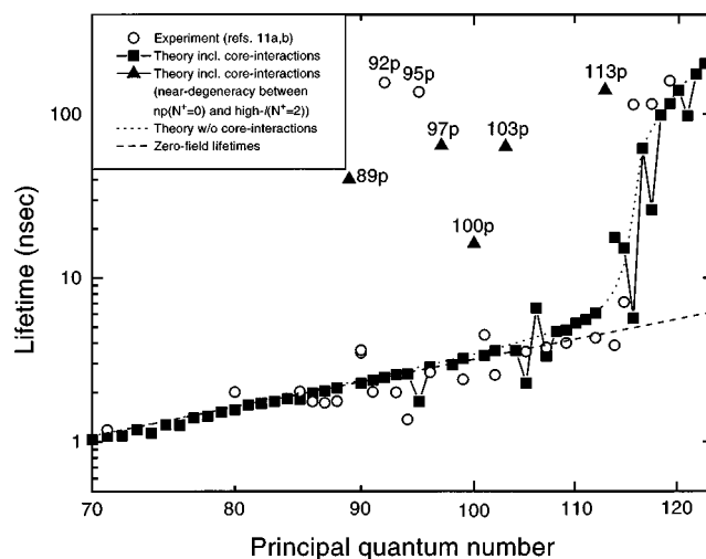
FIG. 6. Calculated (■) and experimental (○) lifetimes of the np(N^+=0) Rydberg series. The calculations were performed for a dc electric field strength of 70 mV/cm. The dashed line shows the natural (zero field) lifetime of the unperturbed np(N^+=0) levels. The dotted line represents the result of a calculation using a field of 60 mV/cm in which the matrix elements representing core interactions ( H_{\text{core}} and H_{sd} ) were suppressed. Special points labeled (▲) are results of the calculations including core interactions where the lifetimes of the np(N^+=0) series members are enhanced via coupling to the nearly degenerate high- l manifold of a Rydberg series converging on N^+=2 .
