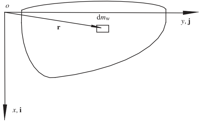
Fig. 3. Diagram showing how the moments and product of inertia are computed. o, x, y , coordinates in wing-fixed frame of reference; dm_w , mass element of the wing; \mathbf{r} , vector distance between point o and a mass element of the wing; \mathbf{i}, \mathbf{j} , unit vectors in the x and y directions, respectively.
