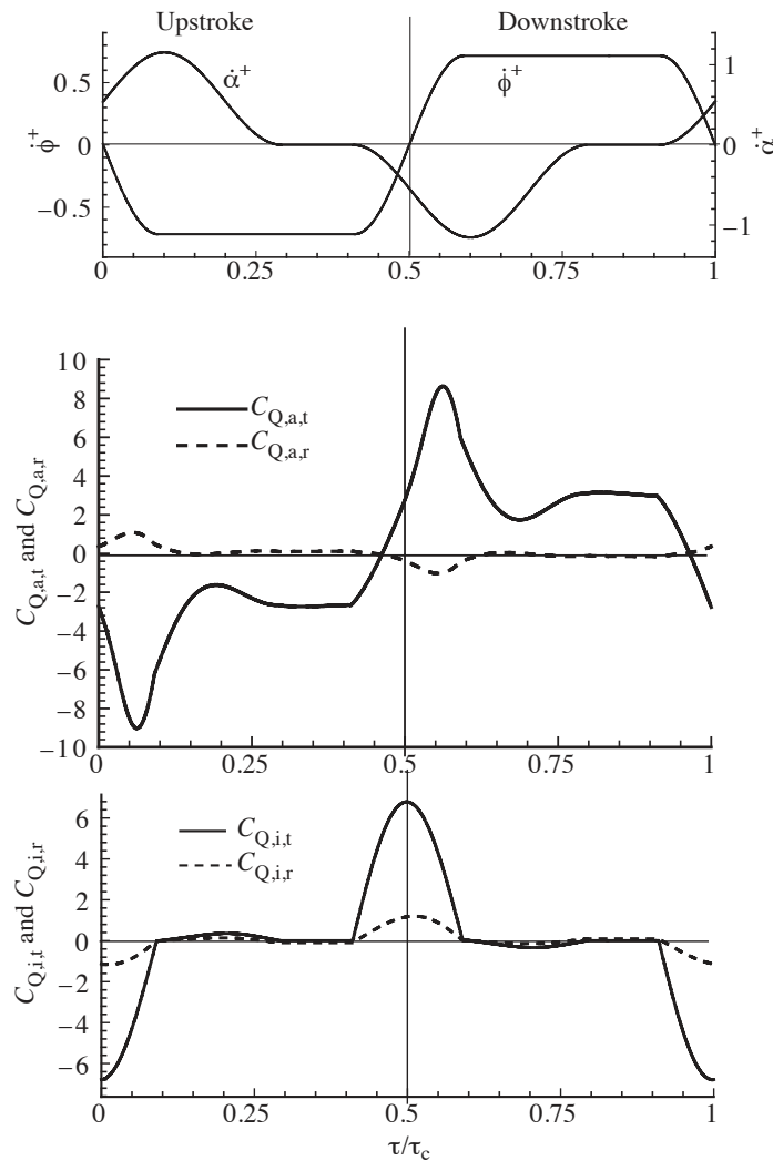
Fig. 11. Non-dimensional angular velocity of pitching rotation \dot{\alpha}^+ and azimuthal rotation \dot{\phi}^+ (A), aerodynamic (B) and inertial (C) torque coefficients for translation ( C_{Q,a,t} and C_{Q,i,t} , respectively) and rotation ( C_{Q,a,r} and C_{Q,i,r} , respectively) versus time during one cycle (midstroke angle of attack \alpha_m=35^\circ , delayed rotation, non-dimensional duration of wing rotation \Delta\tau_r=0.36\tau_c ). \tau_c , non-dimensional period of one flapping cycle; \tau , non-dimensional time.
