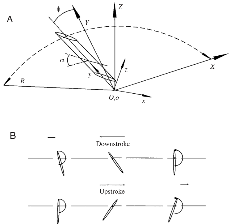
Fig. 1. Sketches of the reference frames and wing motion. (A) OXYZ is an inertial frame, with the XY plane in the stroke plane. oxyz is a frame fixed on the wing, with the x axis along the wing chord, and the y axis along the wing span. \phi is the azimuthal angle of the wing, \alpha is the angle of attack and R is the wing length. (B) The motion of a section of the wing.
