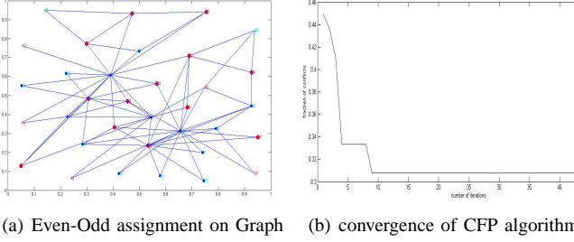
Fig. 2. Even-Odd assignment on Zachary Karate Data [11] using even-odd algorithm 1.
