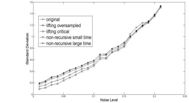
Fig. 5. STD of the original and denoised samples
