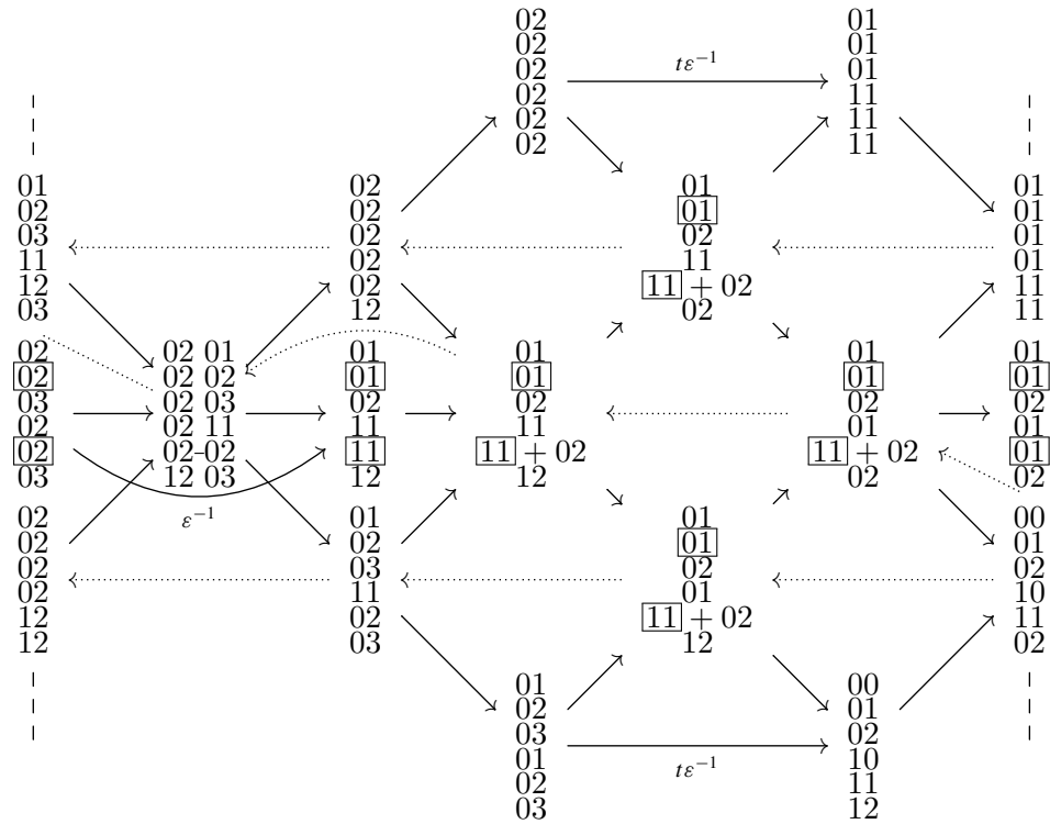
Figure 1. Auslander–Reiten quiver of \text{CM}_e A .
