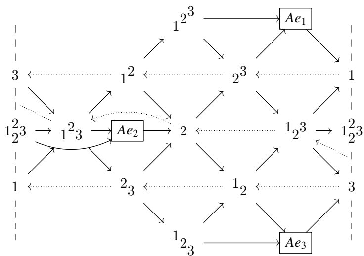
Figure 2. Auslander–Reiten quiver of \text{CM}_e A . Objects are represented by their image by F except objects of add Ae .
