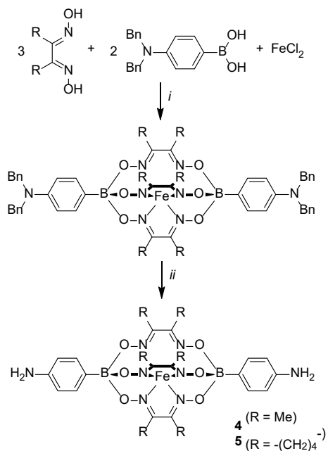
Scheme 5. Synthesis of the clathrochelates 4 and 5 . Reagents and conditions: (i) MeOH, reflux, 4 h; (ii) \text{H}_2 , Pd/C, MeOH/ \text{CHCl}_3 (1.5:1), 50 °C, 4 h.
