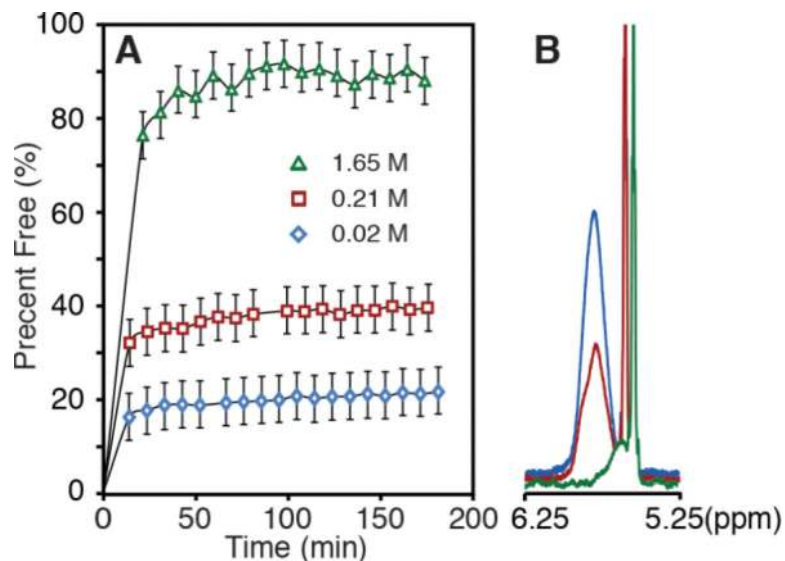
Figure 3. (A) Temporal evolution of (\kappa^2\text{-TMEDA})\text{Cd}(\text{O}_2\text{CR})_2 displacement as measured by ^1\text{H} NMR spectroscopy at several concentrations of added TMEDA in d_6 -benzene. (B) ^1\text{H} NMR spectra of the vinyl region after 200 minutes of reaction. Colors correspond to 0.02 M (blue, diamonds), 0.21 M (red, squares), and 1.65 M (green, triangles) TMEDA solutions. Error bars are set to 10% reflects error in the integration of ^1\text{H} NMR spectra (see experimental).
