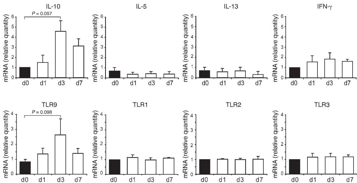
Figure 5 1\alpha25\text{VitD3} elevates IL-10 and TLR9 expression in vivo. \text{CD3}^+\text{CD4}^+ T cells were isolated from 3 steroid-insensitive asthma patients before treatment (d0) and 1, 3, or 7 after treatment with oral calcitriol ( 1\alpha25\text{VitD3} ). TLR and cytokine gene expression was examined ex vivo by real-time RT-PCR. Data are shown normalized to an endogenous control (18S rRNA) and expressed relative to day 0 cells. Mean mRNA levels \pm SEM from 3 donors are depicted.
