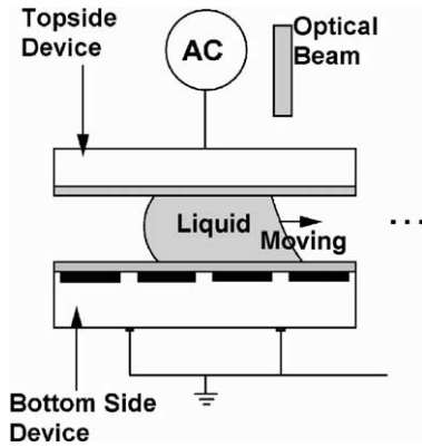
Fig. 3. Principle illustrating light actuation of liquid droplets.
