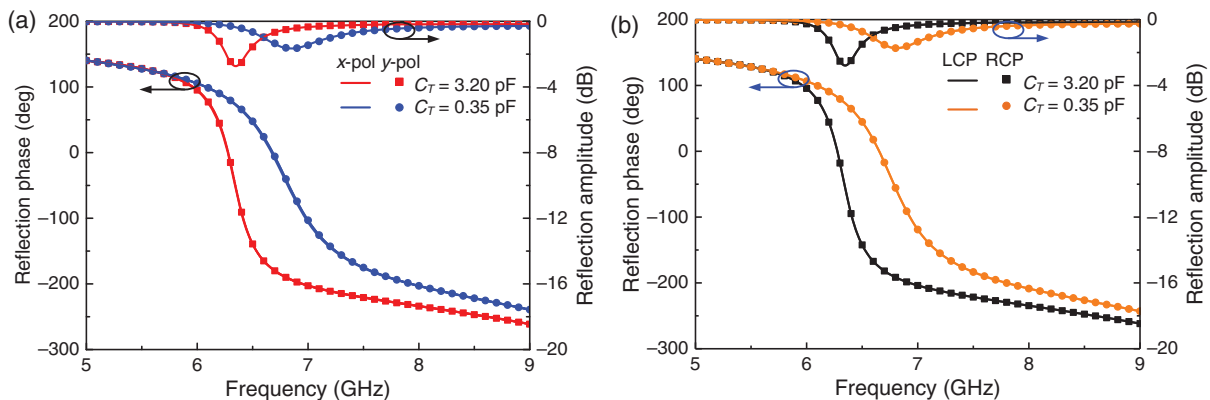
Fig. 2 Reflection performance of the digital metasurface element. (a) Simulated reflection phase and amplitude curves of the element for two different capacitances C_T under x - and y -polarized incidences. (b) Simulated reflection phase and amplitude curves of the element for two different capacitances C_T under LCP and RCP incidences.
