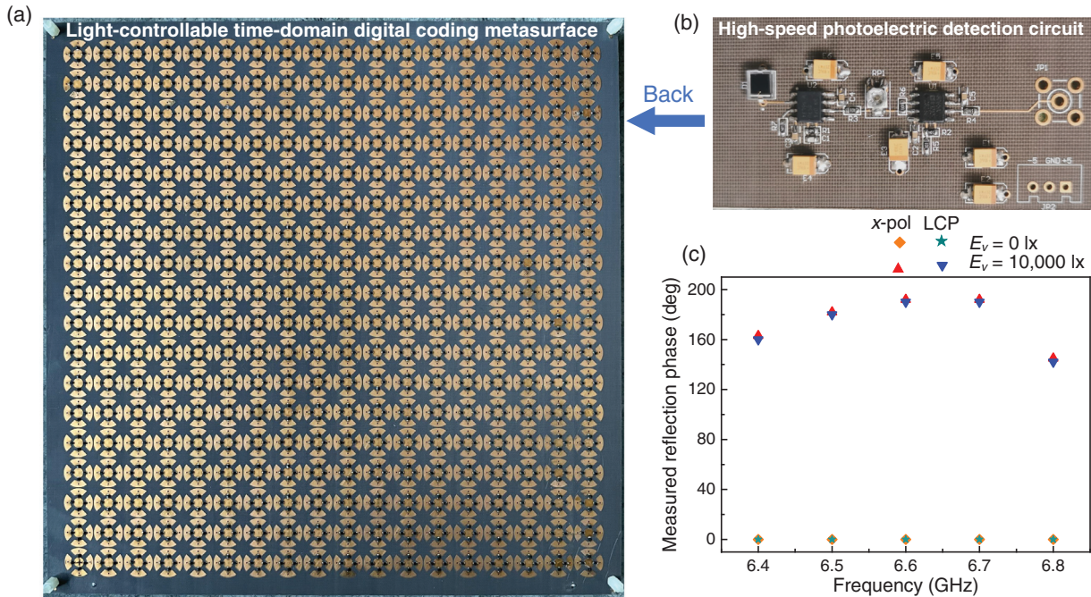
Fig. 3 The fabricated light-controllable time-domain digital coding metasurface and its performance. (a) Photograph of the programmable metasurface sample consisting of 18 \times 18 digital metasurface elements. (b) Photograph of the high-speed photoelectric detection circuit integrated directly into the back of the metasurface sample. (c) Measured reflection phases of the light-controllable metasurface sample at several different frequencies for two different illumination intensities E_v under x -polarized and LCP incidences.
