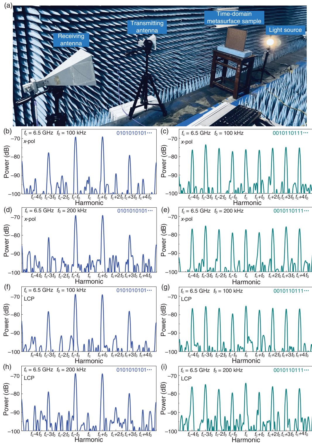
Fig. 4 Experiment setup and tested results. (a) Photograph of the experiment setup for spectrum tests. (b)–(e) Under x -polarized incidences, the measured reflected harmonics of the light-controllable time-domain metasurface at 6.5 GHz for two time-coding sequences of 0101010101... and 0010110111... with different modulation frequencies [(b), (c)] f_0 = 100 kHz and [(d), (e)] f_0 = 200 kHz. (f)–(i) Measured reflected harmonics for corresponding cases under LCP incidences.
