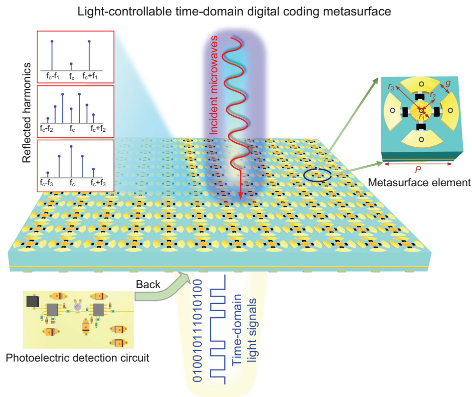
Fig. 1 Schematic of the light-controllable time-domain digital coding metasurface. Such a time-domain metasurface platform is constructed by integrating directly a high-speed photoelectric detection circuit into a full-polarization programmable metasurface. On this hybrid metasurface platform, the microwave reflection spectrum can be manipulated in real time by the light signal with different time-coding sequences.
