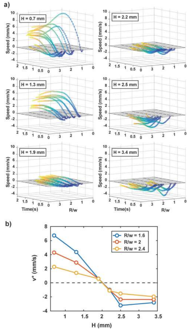
Figure 3. Spatiotemporal analysis of the liquid marble motion shows that the transition between Marangoni and anti Marangoni regimes occurs at H \approx 2 mm. a) Radial speed of a liquid marble upon UV irradiation as a function of time and initial distance to the beam center ( R ) normalized by the beam width ( w ), for various liquid thicknesses ( H ). UV irradiation starts at t = 0 . Lines connecting points are drawn as guides to the eye and indicate the trajectory of a given marble. Marangoni flows are oriented toward the beam center, with a positive or negative speed indicating anti Marangoni or Marangoni behavior, respectively. b) Average speed of the marble ( v^* ) taken in the interval 0.5–1 s as a function of H value for different values of R/w . The horizontal dashed line indicates v^* = 0 .
