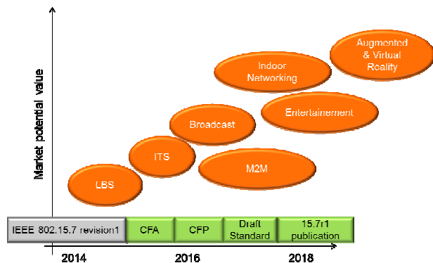
Figure 2. LiFi roadmap
