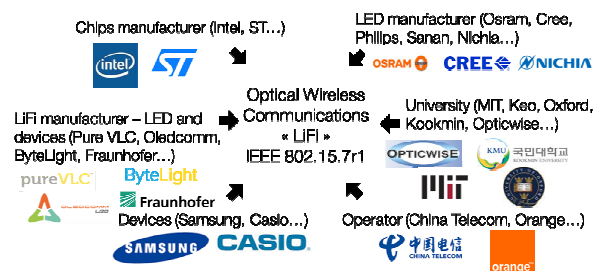
Figure 1. LiFi actors
