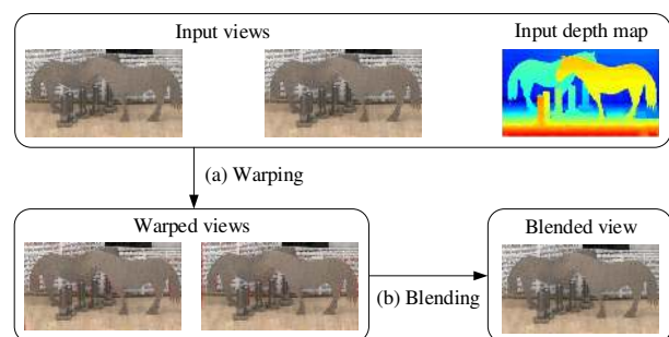
Fig. 10. Typical pipeline of depth image-based view synthesis. (a) Using the input depth map to warp the input images to novel views. In the novel, warped views, the red pixels are blank areas, also called “holes”, caused by the warping operation. (b) Blending the warped views into a single image. The dataset in this figure is the Horses scene from the HCI database [74].
