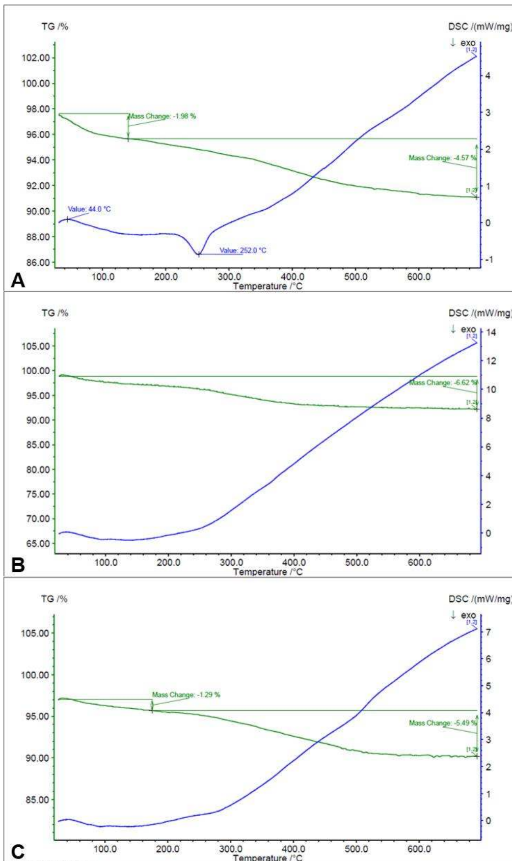
Figure 20. DSC (blue line) and TGA (green line) analysis of the synthetic flavylium 3',4',7-trihydroxyflavylum (A), the dye extracted from the grape waste (B) and the dye extracted from the olive waste (C) adsorbed in the synthesized powder calcined at 400°C. Scan rate equal to 10°C/min.
