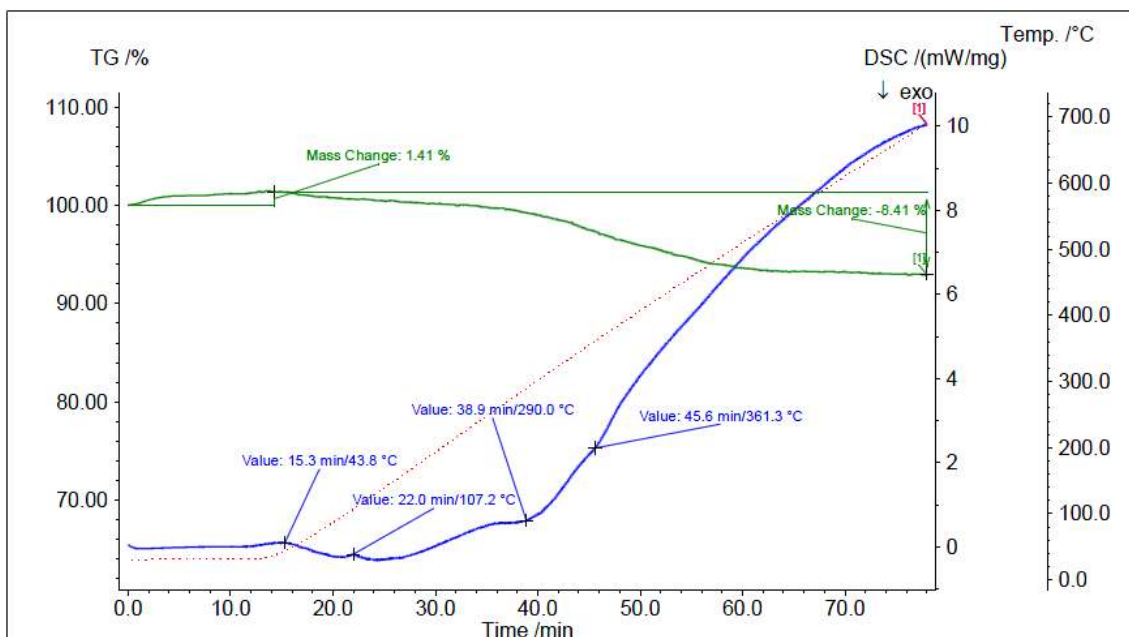
Figure 26. DSC (blue line) and TGA (green line) analysis the \text{TiO}_2 synthesized powder calcined at 400^\circ\text{C} with the dye extracted from the wine waste adsorbed in, after 5 hours of irradiation with a Xe/Hg lamp, at 546 nm. Scan rate equal to 10^\circ\text{C}/\text{min} .
