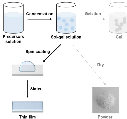
Figure 28. Schematic representation of the \text{TiO}_2 thin film synthesis.
