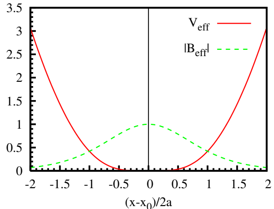
FIG. 2: (Color online) Effective trapping potential V_{\text{eff}} and effective magnetic field B_{\text{eff}} produced by counter-propagating Gaussian beams. The external harmonic potential V_{\text{ext}} cancels the quadratic term in the overall potential V_{\text{eff}} . The effective magnetic field is plotted in the units of B_{\text{eff}}(0) \equiv \hbar k/4a , whereas the effective trapping potential is plotted in the units of \hbar\omega_{\text{rec}}(1 + 1/4a^2 k^2) , with \omega_{\text{rec}} = \hbar k^2/2m .
