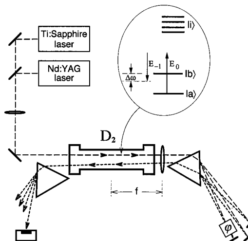
FIG. 1. Experimental setup and energy-level diagram for collinear Raman generation, synthesis of FM and AM light, and detection of the modulation.
