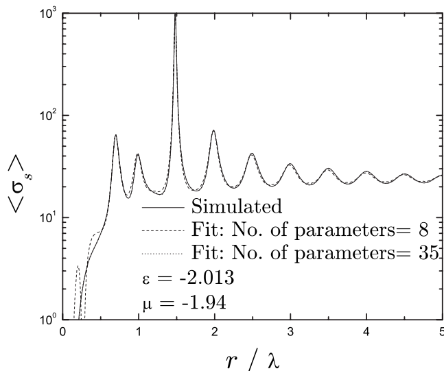
FIG. 5. As in Fig. 3 but with \mu = -1.94 .
