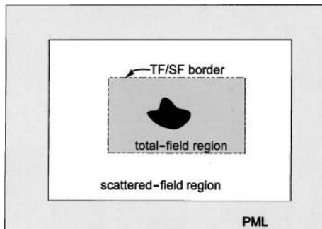
Fig. 4. Regions used by the FDTD method.
