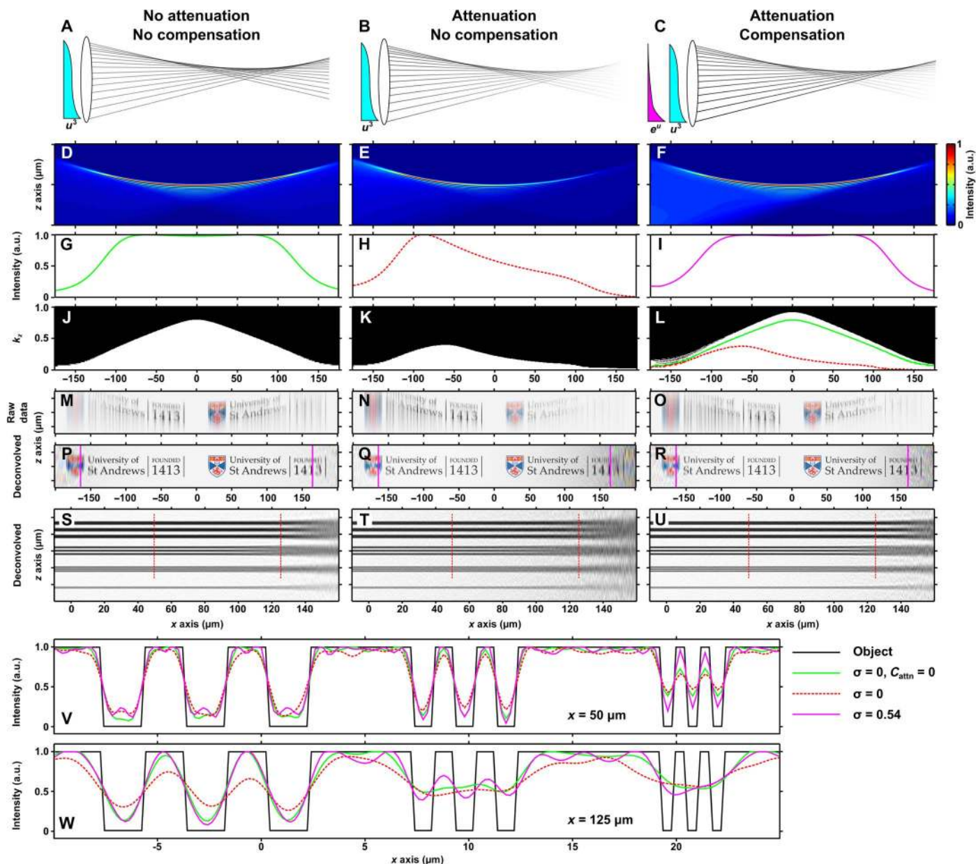
Fig. 1. Principle of attenuation-compensation for an Airy light sheet. Ray optics representations of Airy light-sheet formation without (A) and with (B) attenuation ( C_{\text{attn}} = 65 \text{ cm}^{-1} ) and with attenuation-compensation (C; \sigma = 0.54 ). (D to F) Wave optical simulations of light-sheet profiles, (G to I) peak transverse intensity as a function of longitudinal coordinate, and (J to L) axial MTF thresholded at 5% contrast, respectively, for the light sheets shown in (A) to (C). Green and red lines in (L) match the 5% contour in (J) and (K), respectively. a.u., arbitrary units. (M to R) Simulated, recorded, and deconvolved images of the University crest and (S to U) simulated deconvolved images of a 1D resolution target, respectively, for the light sheets shown in (A) to (C). Pink solid lines in (P) to (R) indicate the edge of the FOV from theory. One-dimensional resolution target (P to R) has linewidth/spacing: 2 \mu\text{m} (top) and 1, 0.6, and 0.2 \mu\text{m} (bottom). (V and W) Intensity profiles through the dashed lines at x = 50 and 125 \mu\text{m} in (S) to (U). Simulation parameters were set to mirror experimental parameters (see Materials and Methods).
