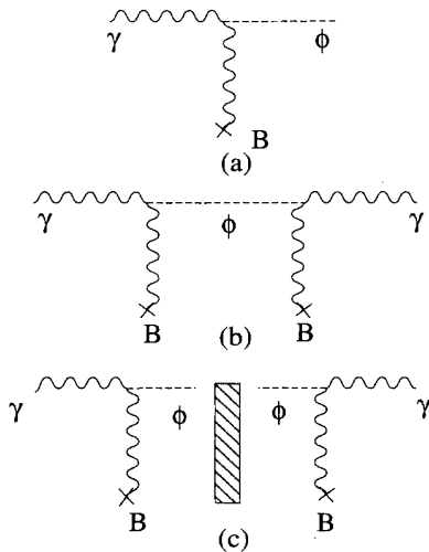
FIG. 3. Diagrams contributing to (a) rotation, (b) ellipticity, and (c) photon regeneration effects of the laser experiments.
