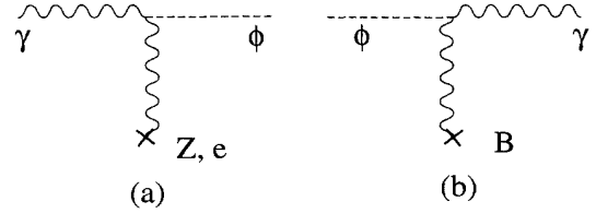
FIG. 4. (a) \phi are produced in the Sun and (b) reconverted in x rays.
