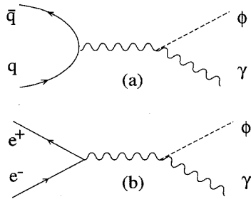
FIG. 1. (a) Diagram of quarkonium decay into \phi and a photon. (b) Diagram of e^+e^- annihilation into \phi and a photon.
