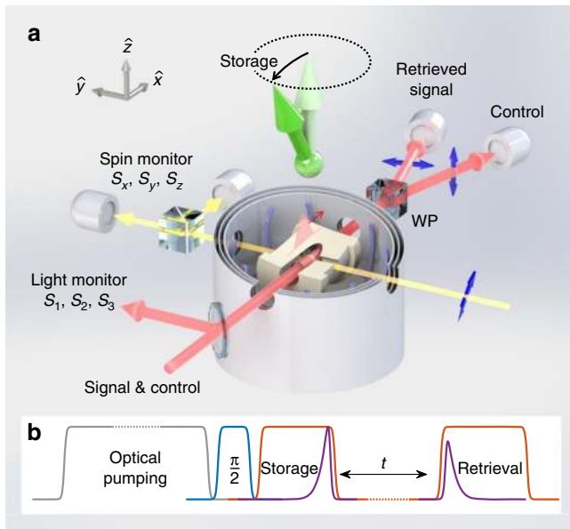
Fig. 2 Experimental setup and sequence. A cylindrical vapor cell with diameter 10 mm and length 30 mm is held inside a hot-air oven ( a , beige), enclosed by three Helmholtz coil pairs and magnetic shield layers. First, optical pumping ( b , gray) is done along \hat{x} using two circularly-polarized beams (not shown in a ) for the two hyperfine sublevels. Subsequently, a \pi/2 pulse of magnetic field along \hat{y} ( b , blue) prepares a spin ensemble oriented along \hat{z} ( a , light green arrow). The control and incoming signal ( a , red beam) are sampled before the cell to monitor their polarization state. Storage and retrieval of a signal pulse ( b , purple) is done by turning off and then on the control ( b , red). The light state is stored onto the orientation of the tilted spin polarization ( a , dark green arrow), which can be monitored with auxiliary far-detuned light ( a , yellow beam). The retrieved signal is separated from the control using a high extinction-ratio Wollaston prism (WP). Blue arrows in a indicate optical polarizations
