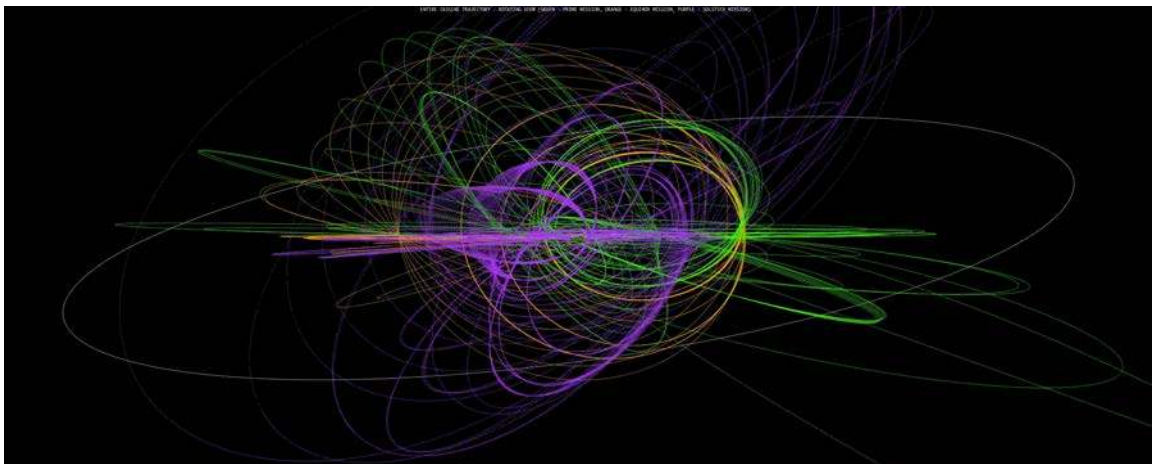
Figure 31. Nonlinear trajectories in the Cassini-Huygen’s space mission: (a) The earth-moon fly-by of the Cassini spacecraft gave a 5.5 km/second speed boost, so although the craft was once again only 1,100 km from Earth after almost 2 years of travel, its speed was considerably greater . (b) Mission planners referred to the trajectories of Cassini as “the ball of yarn”. All orbits between July 1, 2004 and September 15, 2017 are shown in this image. Cassini’s mission terminated in September, 2017. Credit: NASA.
