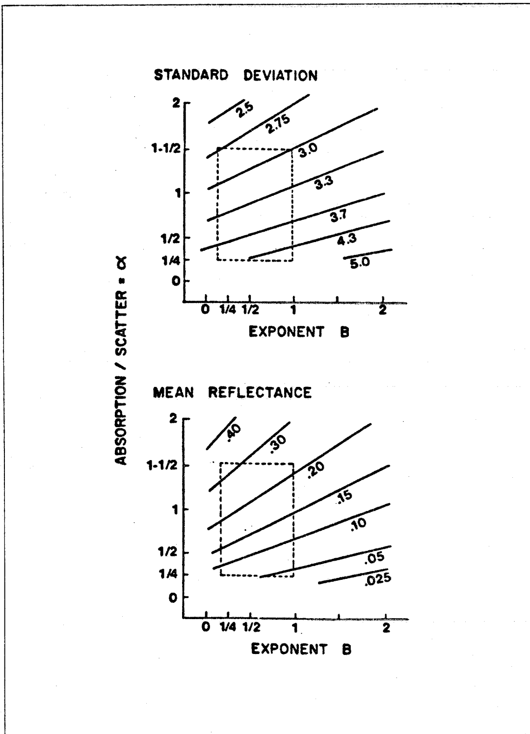
Figure A2. Effect of variations of the two parameters \alpha , \beta on the mean and standard deviation of the probability density function of reflectances as derived from the Kubelka-Munk theory. The practical range of \alpha and \beta is indicated by the dashed rectangle. Note that over this range, the standard deviation of the distribution does not change appreciably.
