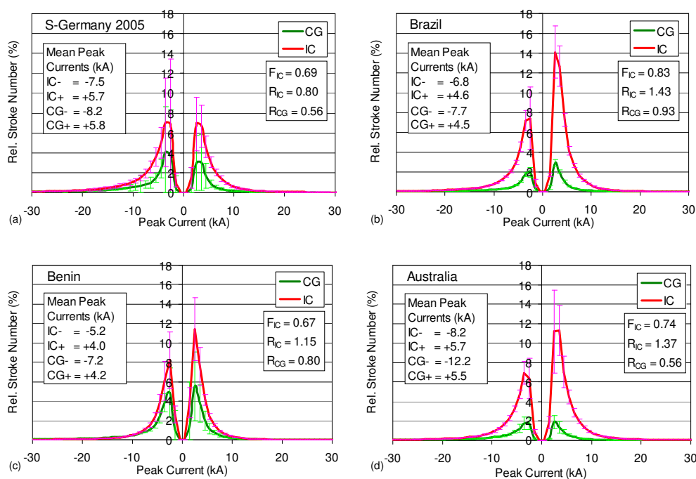
Fig. 28. Number of CG and IC strokes relative to the total number of strokes CG+IC in the respective inner observation region (I) as a function of peak current for (a) S-Germany, (b) Brazil, (c) Benin, (d) N-Australia.
