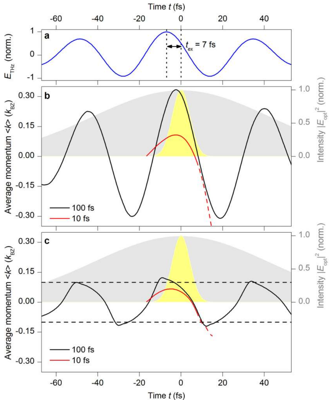
Extended data Figure 6. Influence of excitation-induced dephasing.
