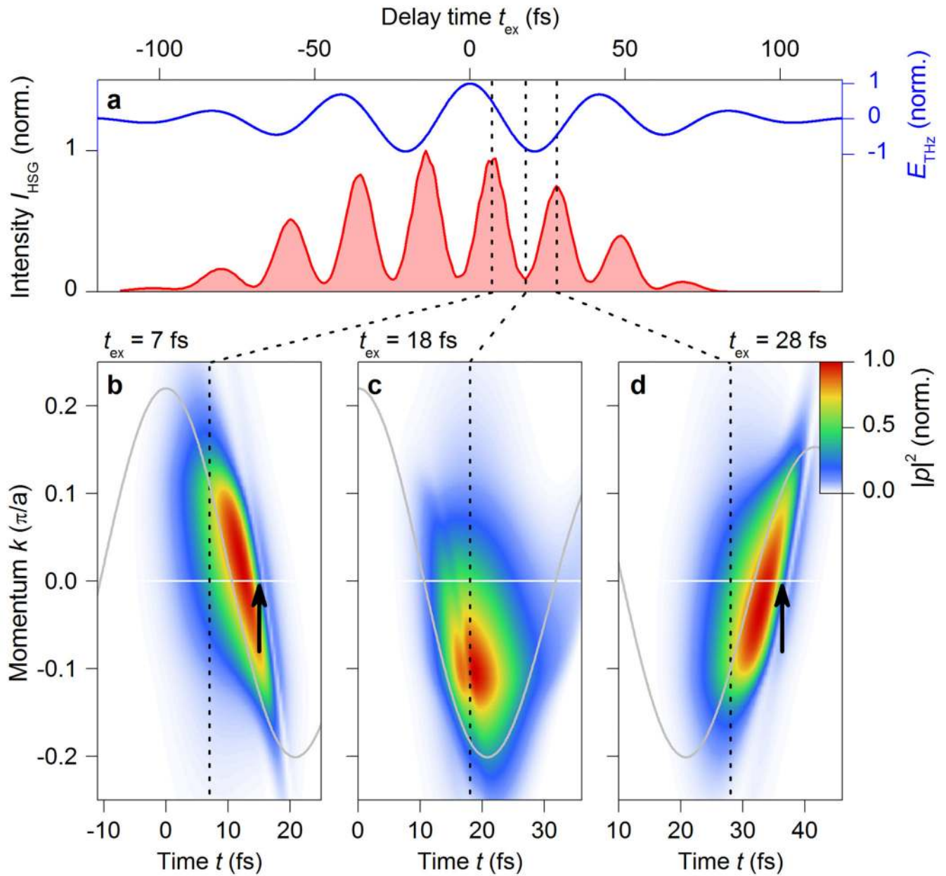
Extended data Figure 3. Coherent excitonic polarization dynamics in k-space.
