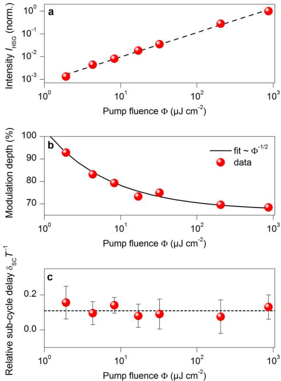
Extended data Figure 2. Pump fluence dependence of time-resolved high-order sideband generation.
