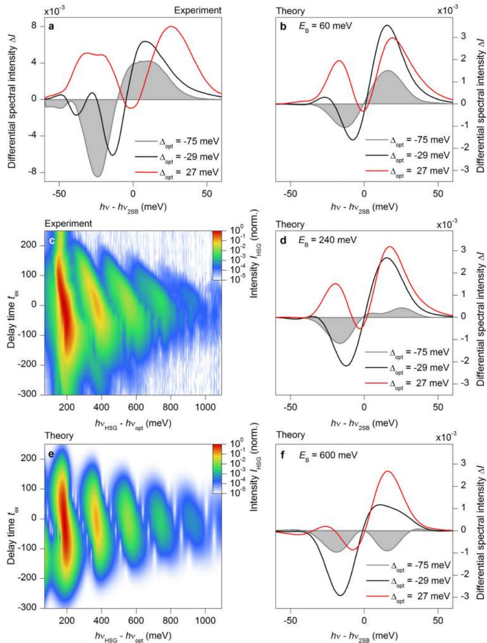
Extended data Figure 9. Quantitative analysis of the binding energy.
