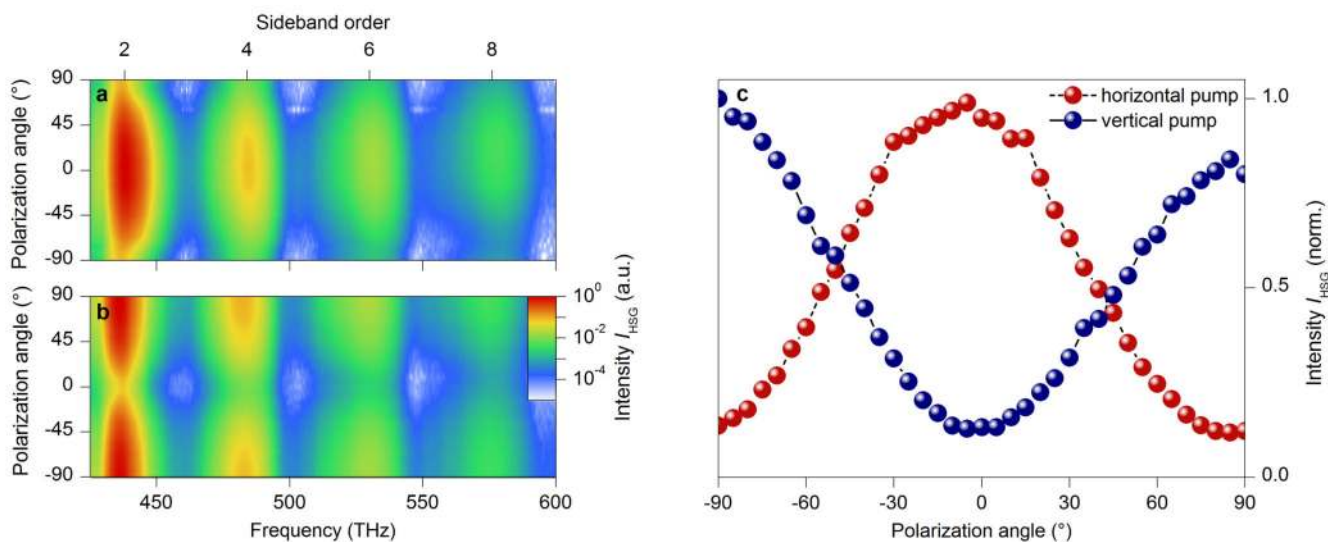
Extended data Figure 1. Polarization of high-order sidebands.
