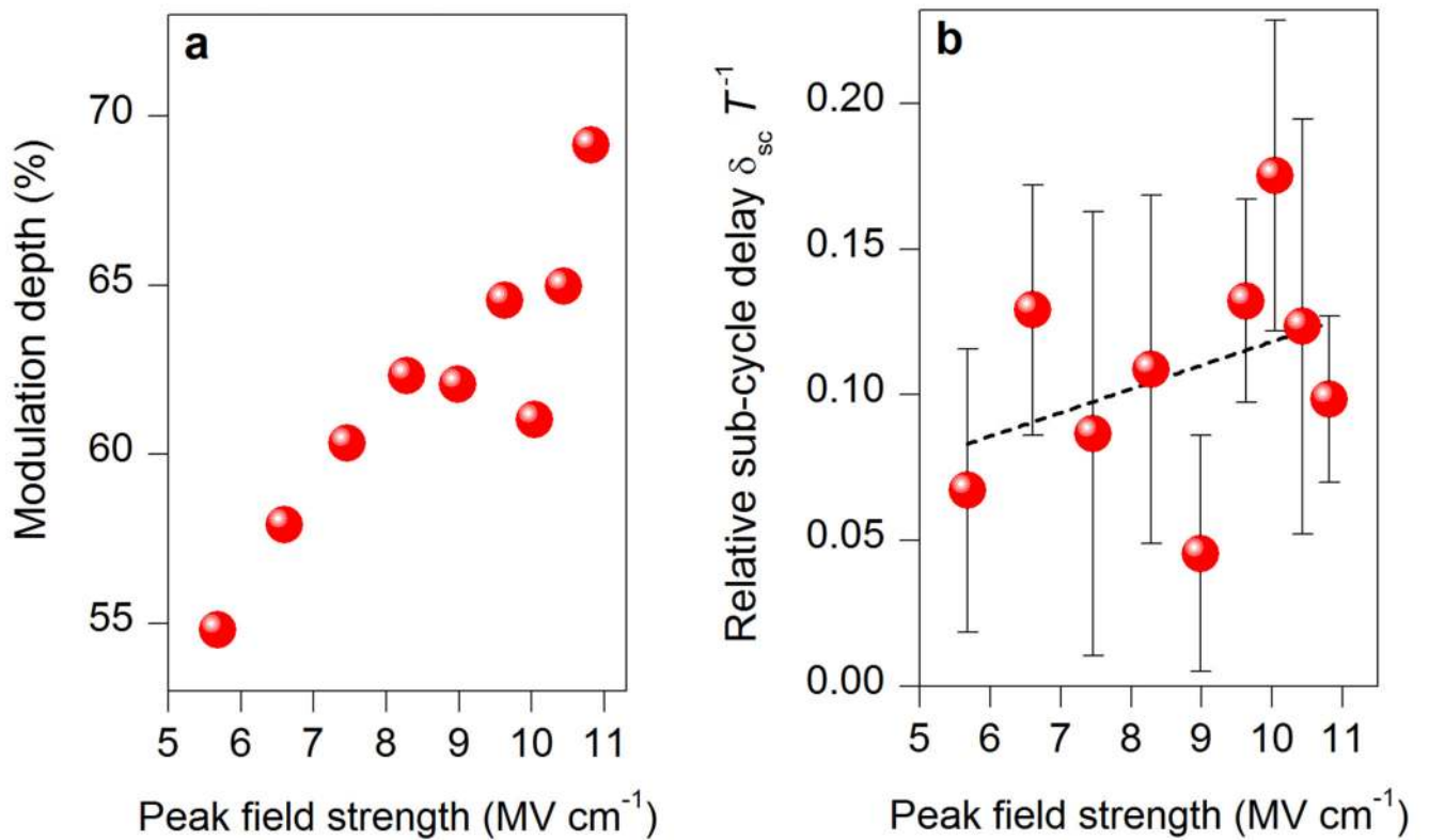
Extended data Figure 5. Field scaling of time-resolved high-order sideband generation.
