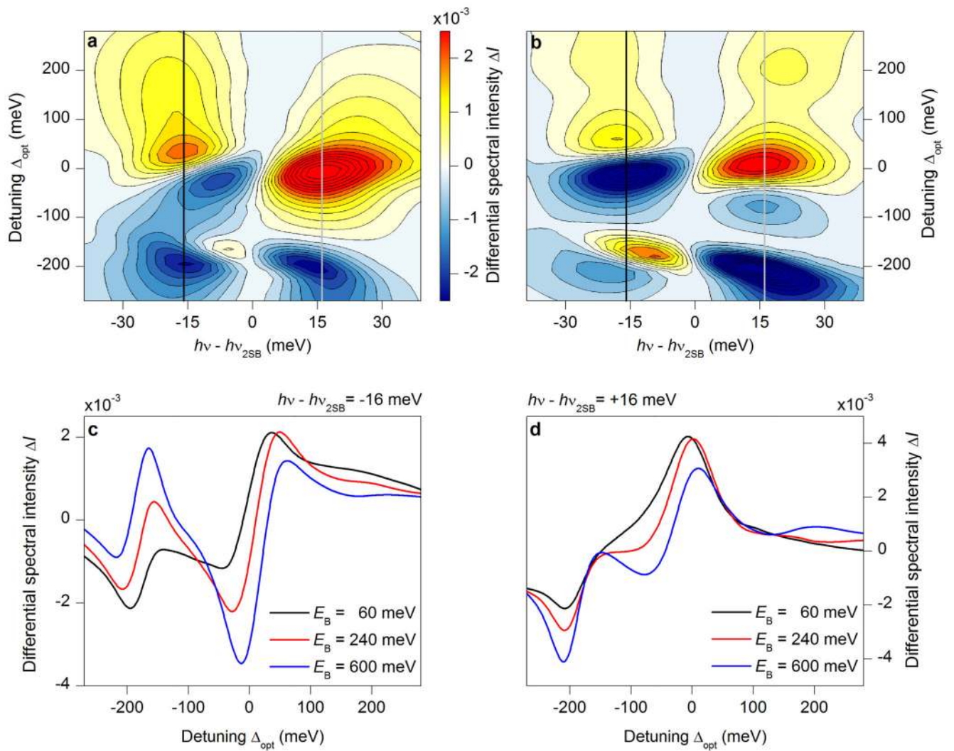
Extended data Figure 8. Differential sideband spectroscopy.
