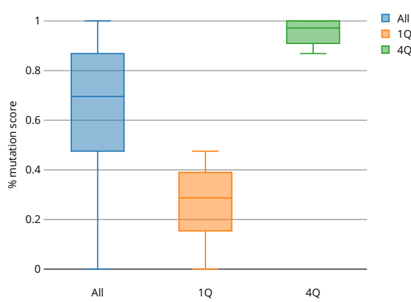
Fig. 1. Distribution of the mutation score for the entire set, the first (non-effective tests) and the fourth quartile (effective tests).
