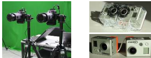
Figure 10: The set-ups used in our experiments. From left to right: A pair of Canon EOS 550D cameras, the GoPro 3D Hero system.
