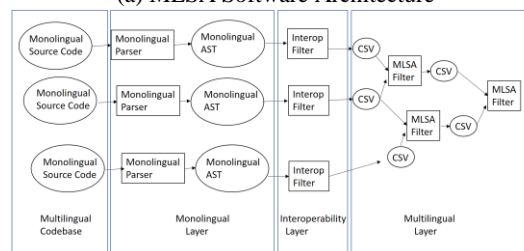
(b) Example MLSA Dataflow
