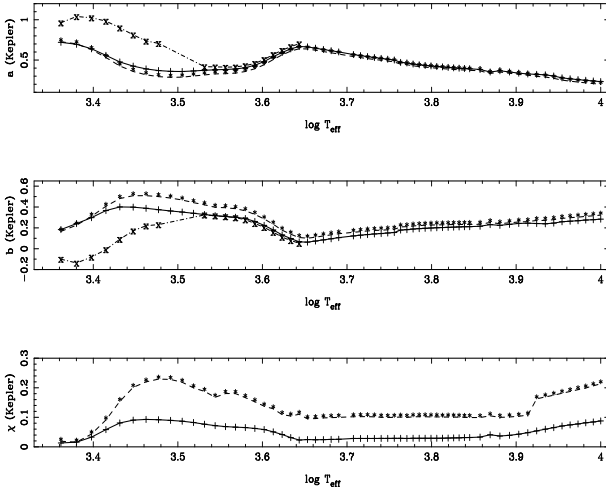
Fig. 1. Quadratic LDC for PHOENIX-COND models. Quasi-spherical models are represented by a continuous line and crosses and the r method by a dashed line and asterisks. The LDC for the PHOENIX-DRIFT models from Claret et al. (2012) are denoted by a dashed-dotted line and the symbol x . In the last case and for the sake of clarity, only models with T_{\text{eff}} < 4400 K are shown. The third panel shows the root square of the merit function \chi . All calculations were performed for \log g = 4.5 , \log[A/H] = 0.0 , V_{\xi} = 2 \text{ km s}^{-1} . Kepler photometric system. LSM calculations.
