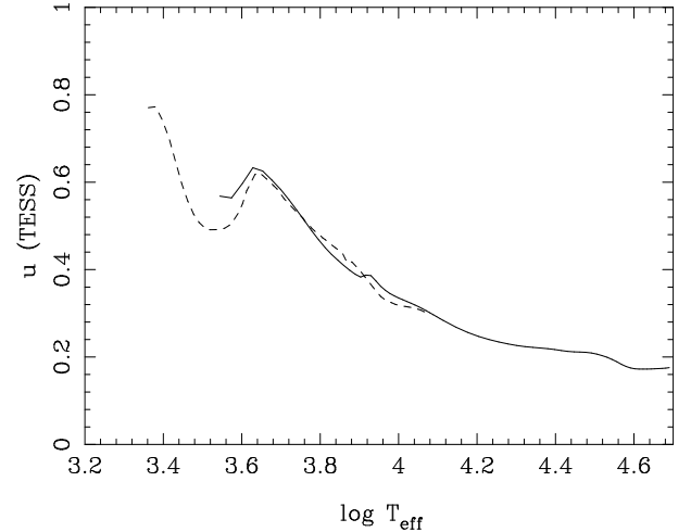
Fig. 2. Theoretical linear LDC for ATLAS models (continuous line) and PHOENIX-COND quasi-spherical ones (dashed line); \log g = 4.5 , \log[A/H] = 0.0 , V_{\xi} = 2 \text{ km s}^{-1} ; TESS photometric system; LSM calculations.
