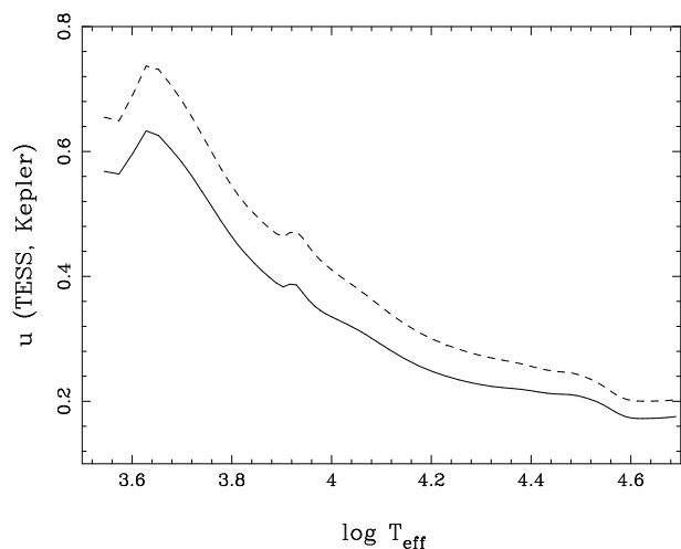
Fig. 4. Theoretical linear LDC for ATLAS models. Continuous line denotes TESS while dashed line represents the Kepler photometric system; \log g = 4.5 , \log[A/H] = 0.0 , V_{\xi} = 2 \text{ km s}^{-1} ; LSM calculations.
