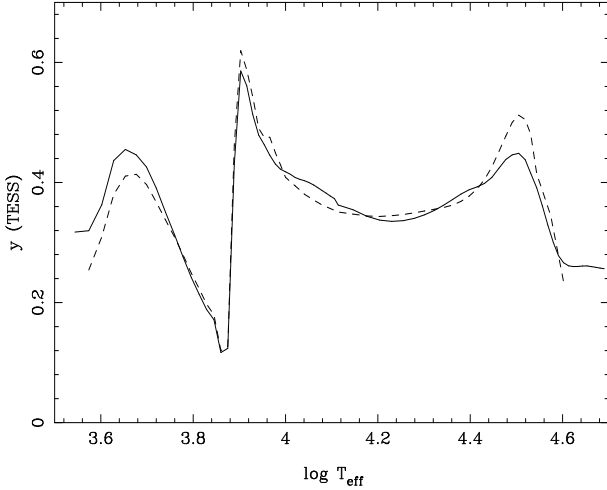
Fig. 6. Theoretical gravity-darkening coefficients for TESS, ATLAS models. The continuous line represents the calculations for \log [A/H] = 0.00 and dashed line is for \log [A/H] = -2.5 , \log g = 4.5 , \log [A/H] = 0.0 , V_\xi = 2 \text{ km s}^{-1} .
