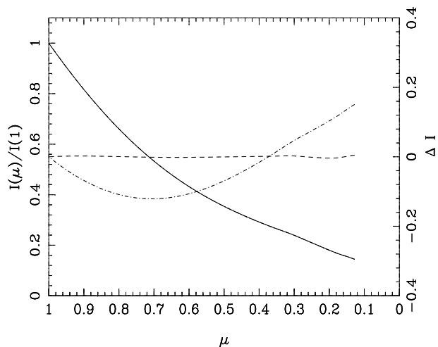
Fig. 3. Specific intensity distribution for a [1500 K, 4.5] PHOENIX-DRIFT quasi-spherical symmetric model. Continuous line represents the model intensities (left label), while the dashed line denotes the deviations [model-fit] by adopting Eq. (5) and the dashed-dotted one represents the deviations by adopting Eq. (1) (right label): \log[A/H] = 0.0 , V_{\xi} = 2 \text{ km s}^{-1} ; TESS photometric system; LSM calculations.
