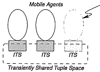
Figure 1: Transiently shared tuple spaces in LIME.
