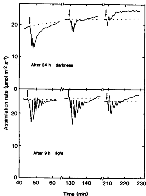
FIG. 3. Response of assimilation rate to 21 mbar O_2 in a leaf kept in darkness for 24 h and for the same leaf at the end of the subsequent 9 h photoperiod. CO_2 was 550 \mu\text{bar} and leaf temp was 15°C. The gas phase was switched from air to 2% O_2 at the arrows. Light intensity was 1500 \mu\text{mol photons m}^{-2} \text{s}^{-1} .
