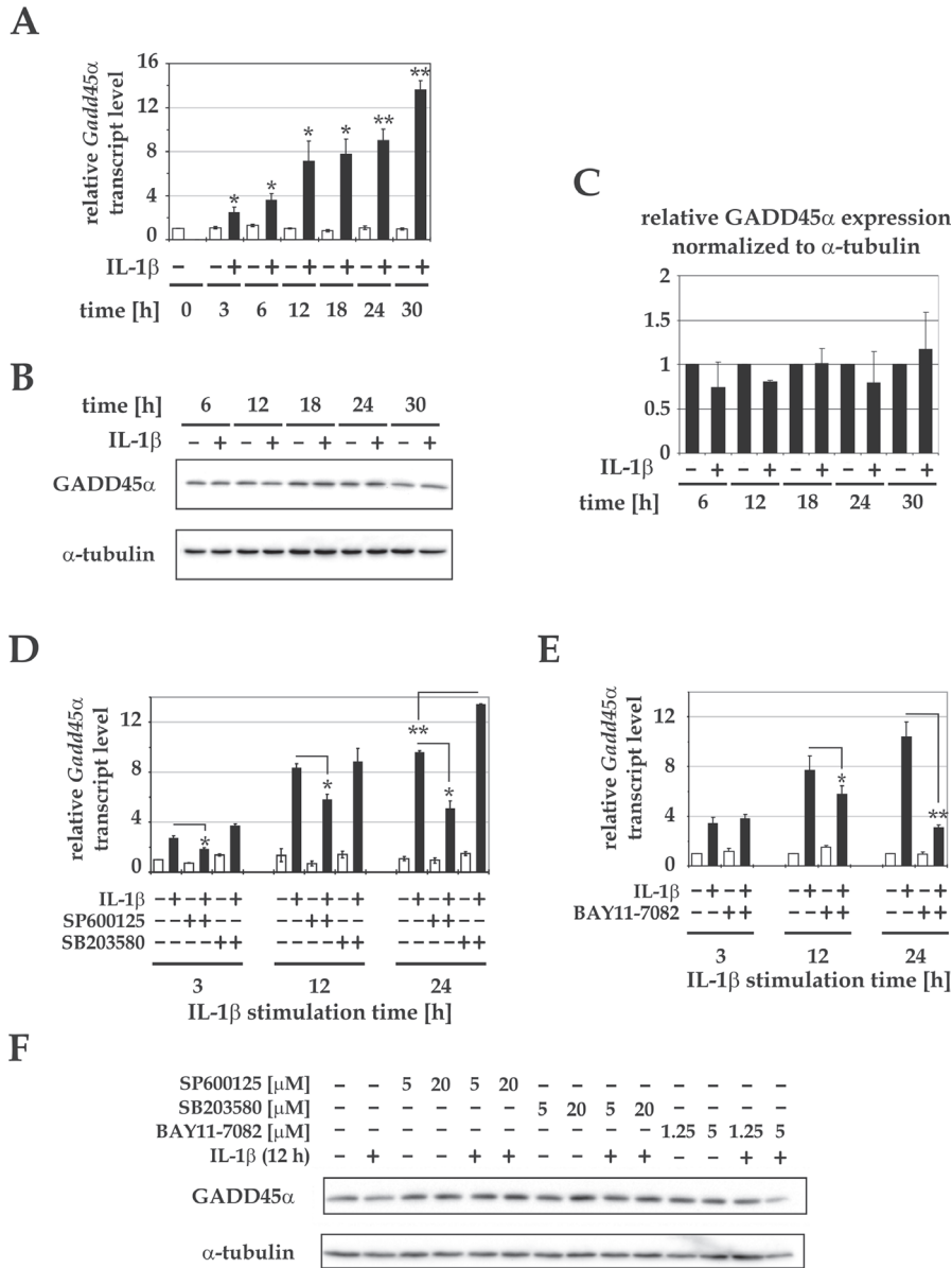
Figure 1. Expression of GADD45α in INS-1E cells after IL-1β stimulation. (A) A real-time PCR analysis of the Gadd45a transcript level time course. Graphs represent the fold-change of the Gadd45a transcript level normalized to untreated cells at the time point "0". (B) Western blot analysis of the time course of the GADD45α protein level. A representative blot from three independent experiments is shown. (C) Densitometry analysis of western blot results from the time course of GADD45α protein, normalized to α-tubulin expression and untreated controls. Shown are means ±S.D. of three experiments. (D) Effect of JNK and p38 inhibition on Gadd45a transcript level after stimulation with IL-1β. The JNK inhibitor (SP600125) and p38 inhibitor (SB203580) were added to the culture medium 1 hour before stimulation and maintained in the medium for the stimulation period. (E) Effect of NF-κB inhibition on Gadd45a transcript level after stimulation with IL-1β. The NF-κB inhibitor (BAY11-7082) was added to the culture medium 1 hour before stimulation and removed prior to IL-1β addition. (F) Effect of JNK, p38 and NF-κB inhibition on GADD45α protein level. A representative blot from three independent experiments is shown. Data points in graphs A, D and E are presented as fold stimulation normalized to untreated controls (graph A) or untreated controls at the time point "3 h" (graphs C and D). The culture media from experiments presented in Fig. 1D and E were used for nitrite accumulation measurements (Fig. 2D and E, respectively). The results presented in graphs A, D and E are means ±S.D. of three experiments. Student's t-test was used for statistical analyses: * p <0.5, ** p <0.01.
