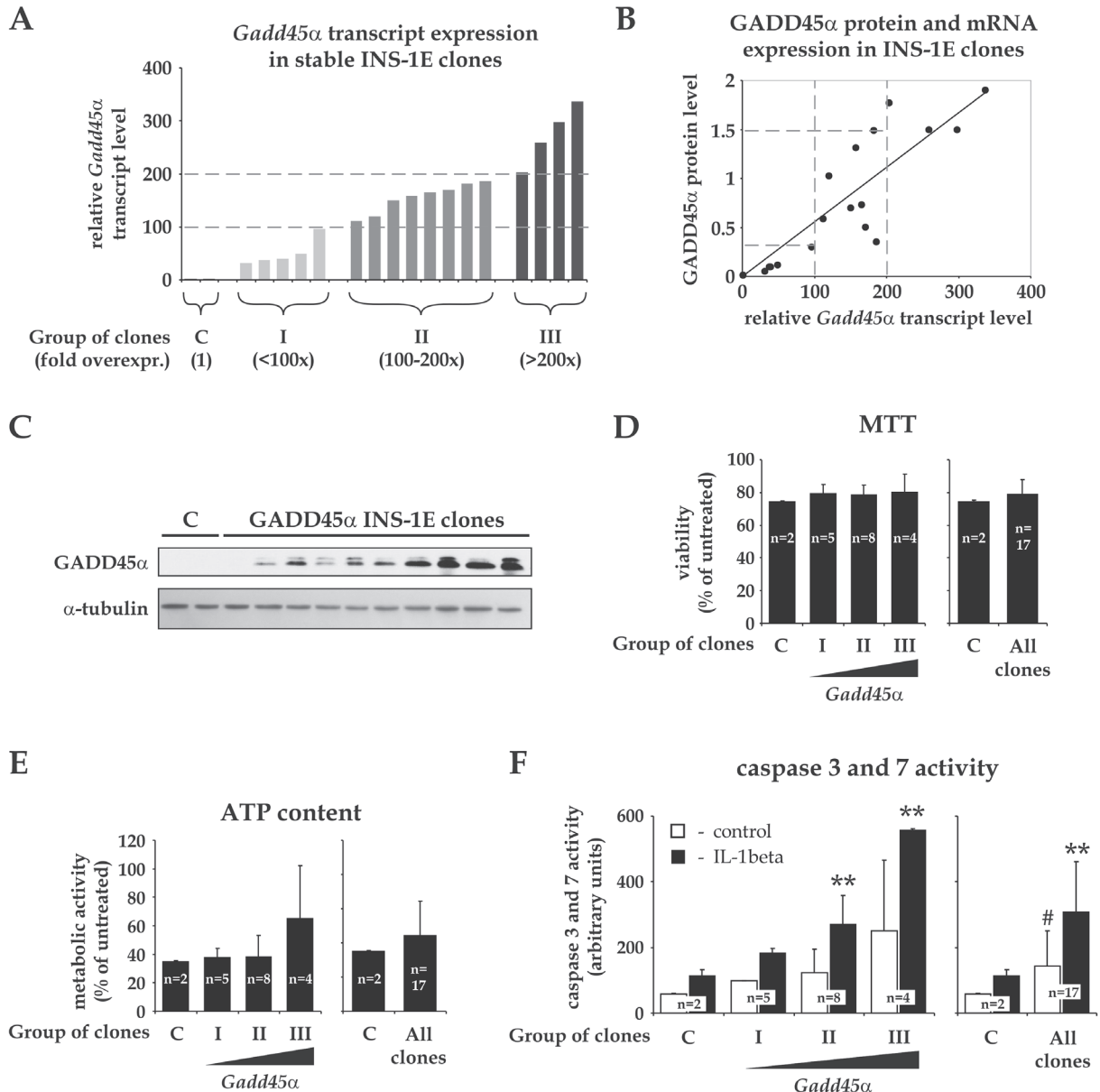
Figure 3. The influence of stable overexpression of GADD45 \alpha on the IL-1 \beta -induced INS-1E cell death.
