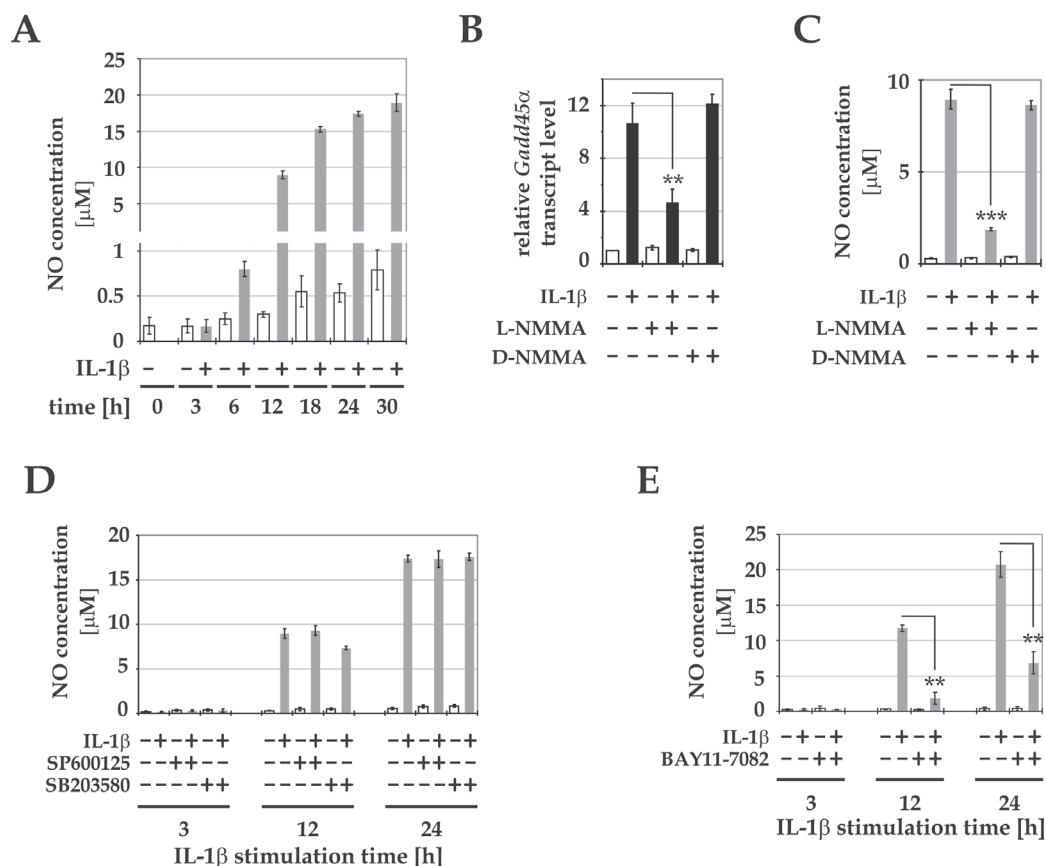
Figure 2. The engagement of nitric oxide in the regulation of Gadd45a expression in INS-1E cells following IL-1 \beta stimulation.
