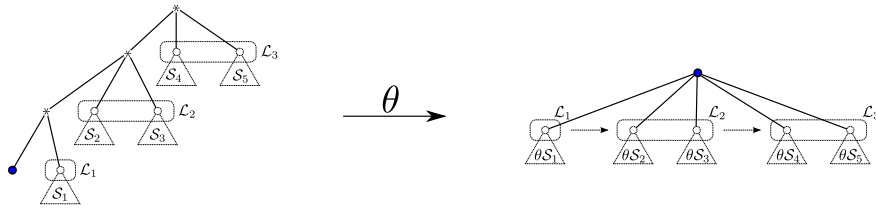
FIG 5. The Ehrenborg–Méndez transformation of Schröder (\mathcal{X} \cdot \mathcal{L}) -enriched parenthesisations into \text{SEQ} \circ \mathcal{L} -enriched trees.
