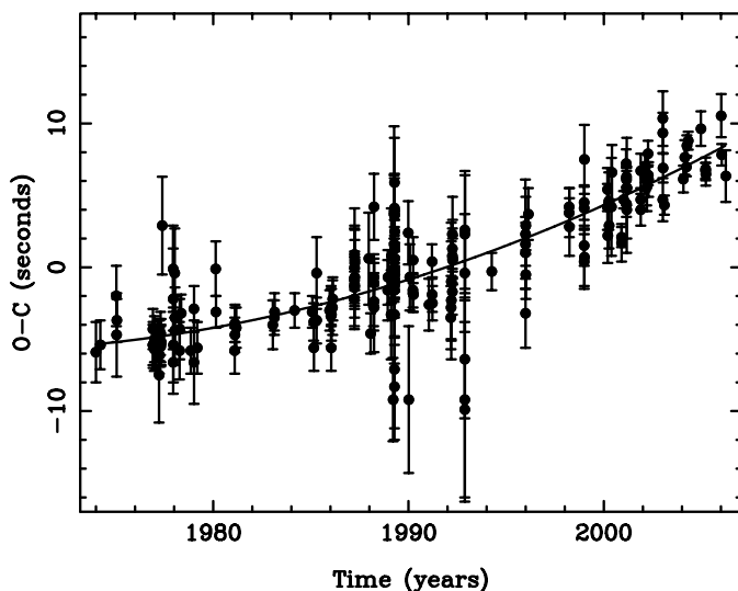
FIG. 4.— Left : The O-C diagram of G117-B15A. Each point represents the phase of pulsation based on a single night of data. The solid line is a parabolic fit to the data. Right : Relief map of the region of parameter space around G117-B15A where we are sensitive to planets. Dark regions indicate a high probability that a planet would have been detected. The large white circles indicate the location of Jupiter and Saturn, while the small circles mark the positions of known extrasolar planets.
