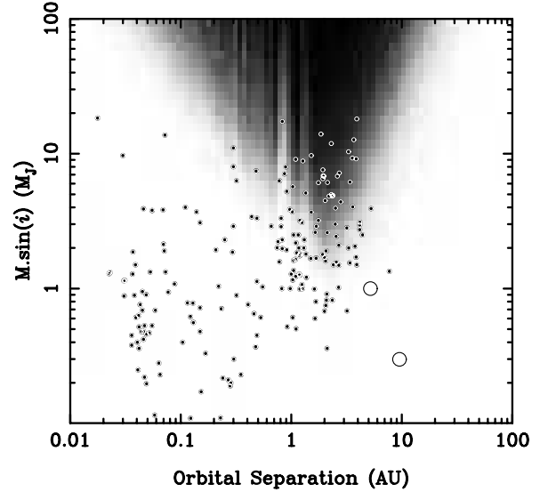
FIG. 7.— Same as Fig. 5, but for GD 244.
