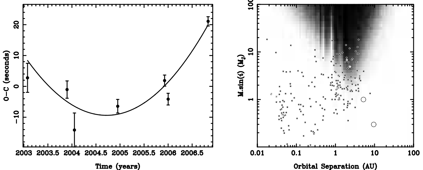
FIG. 10.—Same as Fig. 5, but for SDSS J011100.63+001807.2.
