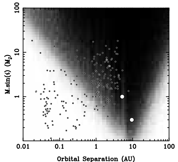
FIG. 4.— Left : The O-C diagram of G117-B15A. Each point represents the phase of pulsation based on a single night of data. The solid line is a parabolic fit to the data. Right : Relief map of the region of parameter space around G117-B15A where we are sensitive to planets. Dark regions indicate a high probability that a planet would have been detected. The large white circles indicate the location of Jupiter and Saturn, while the small circles mark the positions of known extrasolar planets.
