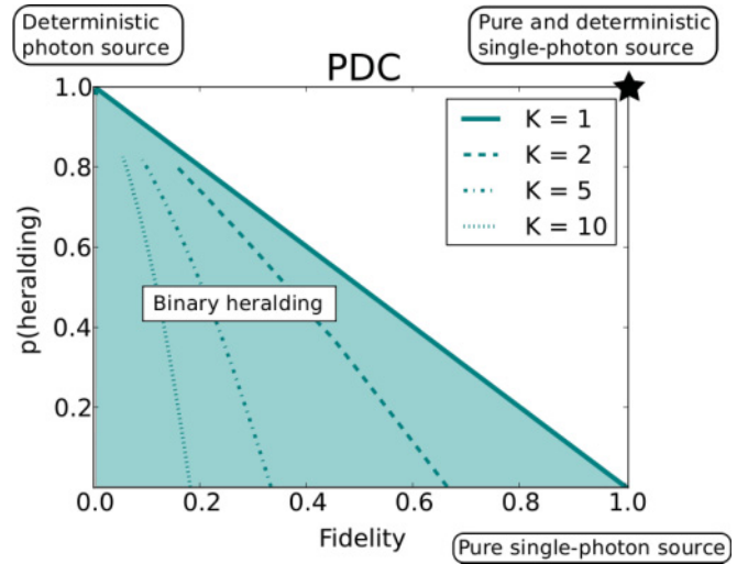
FIG. 4. (Color online) Heralding probabilities, p(\text{heralding}) , and single-photon Fock-state fidelities, Fidelity , of the state created using various multimode PDC sources in conjunction with a binary detector featuring unit detection efficiency \eta = 1 . Multiple frequency modes K = 2, 5, 10 severely limit the achievable maximum fidelities.
