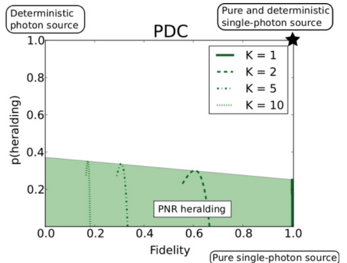
FIG. 5. (Color online) Heralding probabilities, p(\text{heralding}) , and single-photon Fock-state fidelities, Fidelity , of the state created using various multimode PDC sources in conjunction with a photon-number-resolving detector featuring unit detection efficiency \eta = 1 . Again, multiple frequency modes K = 2, 5, 10 severely limit the achievable maximum fidelities.
