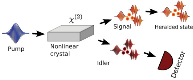
FIG. 1. (Color online) Schematic of the PDC process used to herald single-photon states: An incoming pump pulse decays inside a nonlinear medium into two beams labeled signal and idler which feature a perfect photon-number correlation. The idler beam is subsequently detected to herald the presence of the signal state.
