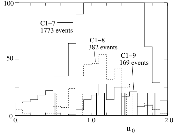
Fig. 6. The u_0 (mean of those for R_{\text{eros}} and B_{\text{eros}} ) distribution for LMC and SMC light curves surviving cuts C1 – C7 , C1 – C8 , and C1 – C9 . The positions of the 14 light curves surviving cuts C1 – C10 are shown with the 4 supernovae as dashed lines.
