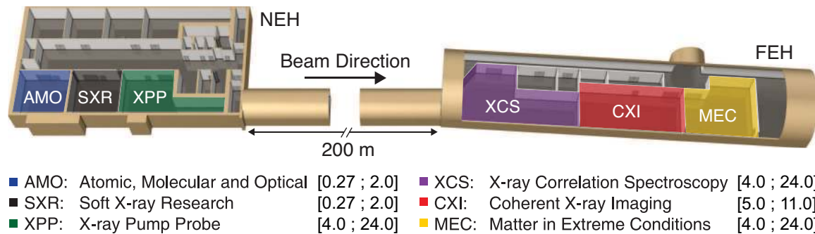
FIG. 8 (Color) The three instruments in the Near Experimental Hall (NEH) were commissioned first in a phased approach starting in October of 2009 with user science experiments on the AMO instrument, followed by SXR in July 2010 and XPP in October 2010. In the Far Experimental Hall (FEH) experiments began on CXI in February 2011 followed by XCS in November 2011 and MEC in April 2012 to form the complete facility. The X-ray energy range in keV is specified for each instrument in brackets. Third harmonic radiation is used for photon energies greater than 12.7 keV.
