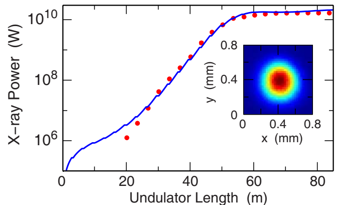
FIG. 3 (Color) Linac Coherent Light Source free-electron laser power (red points) at 1.5 \text{ \AA} versus active undulator length. The measured gain length is 3.3 m and a GENESIS simulation is overlaid in blue with electron beam parameters measured. The X-ray image on the yttrium aluminium garnet screen is shown in the insert. Adapted from Emma et al. , 2010.
