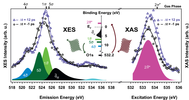
FIG. 35 (Color) Oxygen K-edge X-ray emission spectroscopy (left) and X-ray absorption spectroscopy (right) data of CO/Ru(0001) with corresponding fits (solid lines) for both before the excitation and for 12 ps afterwards. At the bottom, the peak deconvolution resulting from the fit of the spectra is shown, with the elastic peak being indicated in light blue around 534 eV. (Middle) A schematic illustration of the excitation process from the O1s level to the unoccupied 2\pi^* resonance in XAS and the core-hole decay process from occupied molecular orbitals back to the O1s in XES. From Dell'Angela et al. , 2013.
