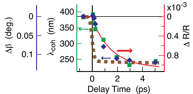
FIG. 22 (Color) Universal curve showing the speed of the metal-to-insulator transition in magnetite. X-ray data (blue/green symbols and dashed brown line) taken at the (0,0,1/2) reflection (Fe L_3 -edge) shown together with the optical reflectivity (red line, representing an exponential fit to the data). The reduction in the electronic ordering coherence length ( \lambda_{coh} , green squares) and the change in diffraction angle ( \Delta\beta , blue diamonds) occur concomitantly with the increase of the optical reflectivity ( \Delta R/R , red curve) with a time constant of 1.5 \pm 0.2 ps. This decay occurs with a delayed onset as clearly indicated by the unchanged \lambda_{coh} and \Delta\beta values at 200 fs time delay and reflects the structural modifications towards the cubic lattice where metallic charge fluctuations reduce the coherence of the remnant patches of electronic order. For comparison: The trimeron lattice diffraction intensity versus time (dashed brown solid line) shows a fast quench, reflecting the time resolution of the experiment. From de Jong et al. , 2013.
