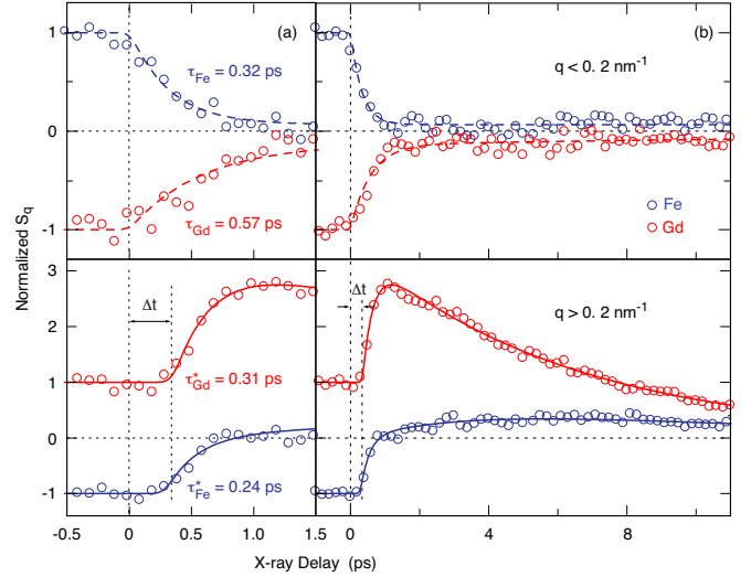
FIG. 25 (Color) Reversal of Gd spins within nanoscale Gd-rich regions as measured by resonant X-ray diffraction. (a) Temporal evolution of the magnetic structure factor, S_q , for Gd 4f spins (red) and Fe 3d spins (blue) measuring the local deviations from the average magnetization. (b) The same S_q data but on a longer timescale. The S_q signals were integrated over the low- q region of the magnetic diffraction pattern ( q < 0.2 \text{ nm}^{-1} ) and high- q ( q > 0.2 \text{ nm}^{-1} ) regions and are normalized to the equilibrium values. Therefore, |S_q(t < 0)| = 1 for both q -ranges and sublattices, although high- q S_q for Gd is \sim 4 times greater than for Fe. Dashed and solid lines represent fits of exponential decay/rise functions to the data. The observed delayed onset at \Delta t = 360 \pm 50 \text{ fs} indicates that angular momentum transfer effectively occurs only after this time delay. Beyond 1 ps, the Gd (Fe) data are well described by an exponential decay (rise) with a time constant of 6 \pm 2 \text{ ps} . The Fe data is fit with an additional decay with time constant 8 ps. From Graves et al. , 2013.
