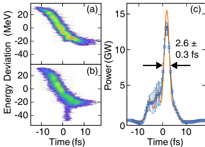
FIG. 5 (Color) X-band deflecting cavity (XTCAV) measurements of sub-5 fs, 1 keV X-ray pulse. The electron bunch charge is 20 pC with electron beam energy of 4.7 GeV. (a) One single-shot lasing-off image; (b) One single-shot lasing-on image; (c) Reconstructed X-ray profile with a calculated 2.6 fs fwhm duration. Adapted from Behrens et al. , 2014.
