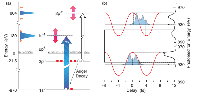
FIG. 15 (Color) Comparison of (a) sideband generation and (b) streaking in mixed optical and X-ray laser fields. Sidebands are symmetrically distributed around the main line and they reflect the exchange of photons from both fields during more than one optical period. In streaking experiments (b) the photoelectrons experience a redistribution of kinetic energy that depends on the magnitude of the electric field at the instance of their generation during a sub-cycle of the optical laser field. Adapted from Dusterer et al. , 2011 and Helml et al. , 2014.
