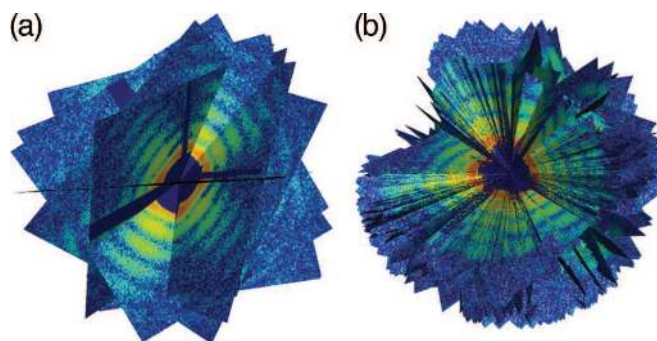
FIG. 44 (Color) Assembled 3-dimensional mimivirus diffraction pattern from 198 2D diffraction patterns. (a) Subset of 10 diffraction patterns shown in their best orientation. (b) All 198 diffraction patterns shown with a cutout showing the origin in reciprocal space. Adapted from Ekeberg et al. , 2015.
