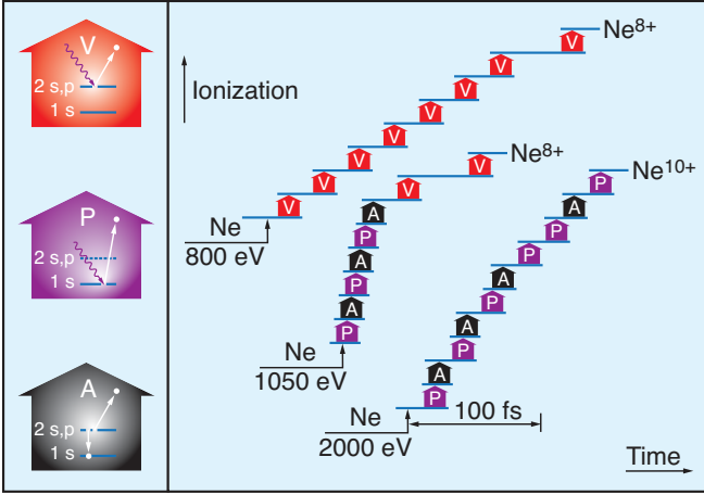
FIG. 9 (Color) Diagram of sequential X-ray multiphoton ionization in neon. The highest possible charge states are the ones energetically accessible by one photon ionization. Below the Ne 1s threshold only valence electrons are ionized (V process); above the threshold, a photoionization (P) and Auger (A) decay processes alternate. For increasing charge states the core-hole lifetimes increase, leading to subsequent photoionization (P - P) processes and X-ray induced X-ray transparency. From Young et al. , 2010.
