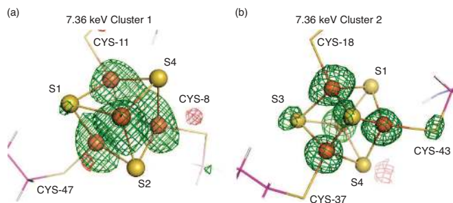
FIG. 43 (Color) Difference electron density between a synchrotron structure and an LCLS high-dose structure in ferredoxin. Clear differences in the electron density are visible from the green positive density and the red negative density contoured at the 3\sigma level. (a) Cluster 1 and (b) Cluster 2 at 7.36 keV. S1, S3 and S4 represent the sulfur atoms labeled 1 to 4 (S3 not shown). The cysteine (CYS) amino acids around the clusters are labeled with the residue number in the protein sequence. Adapted from Nass et al. , 2015.
