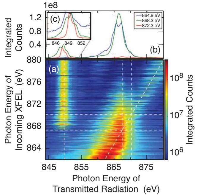
FIG. 18 (Color) Measured single-shot emission spectra as a function of the incoming photon energy (a) and three distinct line-outs with as-measured (b) and normalized (c) intensities. The XFEL pulses appear as a diagonal line in (a) which is heavily attenuated for photon energies above the Ne K-edge at 870 eV. The dominant emission line appears at 850 eV. Below 867.5 eV excitation energy the emission is absent and above 870 eV the line is stable. For the intermediate emission energy regime, the line profile and peak position vary strongly, owing to stimulated electronic X-ray Raman processes. Adapted from Weninger et al. , 2013.
