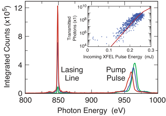
FIG. 17 (Color) X-ray pumped X-ray lasing. Selected single-shot spectra of the neon X-ray lasing line at 850 eV and simultaneously transmitted FEL pulse around 960 eV. The X-ray lasing line width is much narrower and jitter free. Note that the FEL pulse is attenuated by the neon gas by about three orders of magnitude compared to the incoming pulse energy. The inset displays the exponential gain with increasing pump power. Adapted from Rohringer et al. , 2012.
