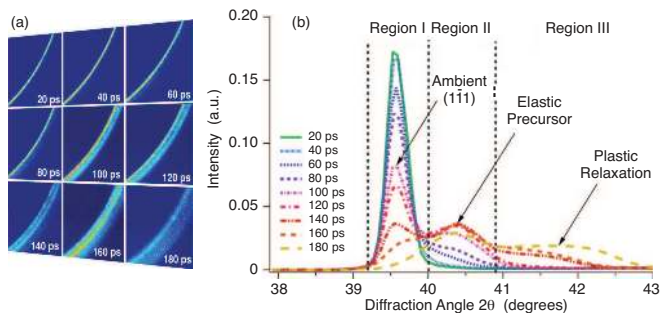
FIG. 30 (Color) (a) A section of Debye-Scherrer ring showing evolution of lattice dynamics with time delay (b) Diffraction profile illustrating the characteristic lattice response. Adapted from Milathianaki et al. , 2013.
