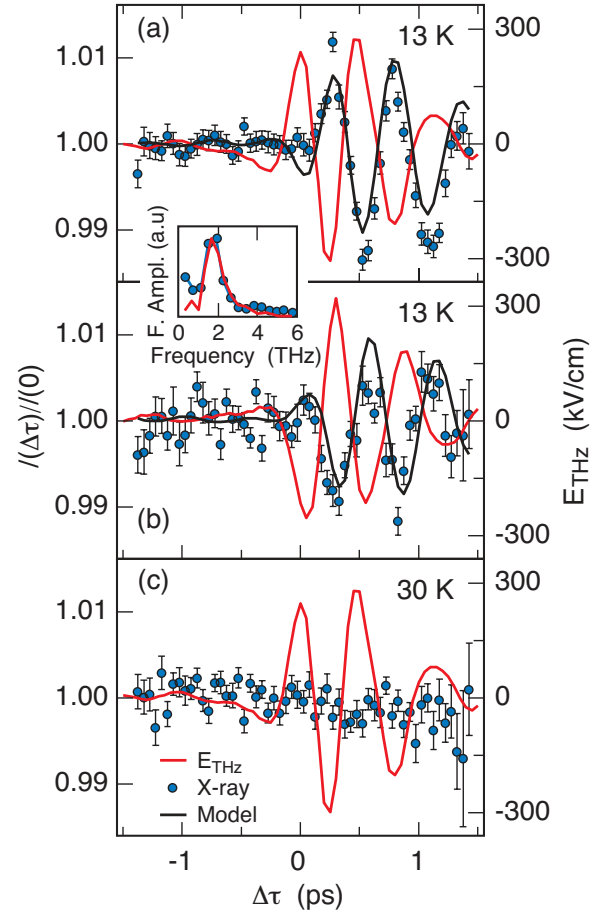
FIG. 24 (Color) Time-dependent behavior of an electromagnon. The magnetic diffraction of the (0k0) peak of \text{TbMnO}_3 (blue symbols) is compared with the electric field of the THz pump (red solid line) as a function of the time delay. (a) The response of the sample in the multiferroic phase at T = 13 K and for (b) an inverted electric field driving pulse. (c) The response for the system in the spin-density wave phase for T = 30 K, where the effect vanishes. From Kubacka et al. , 2014.
