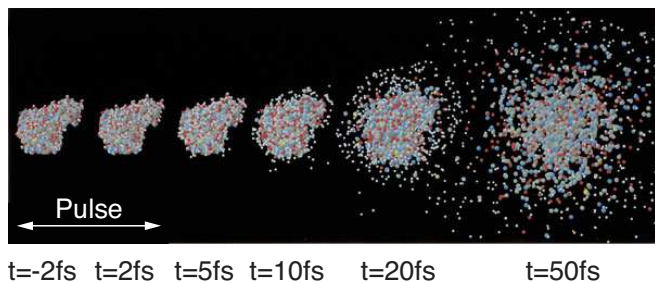
FIG. 6 (Color) Diffraction-before-destruction concept showing how nuclear motions caused by an X-ray FEL pulse can occur primarily after a suitably short pulse has passed through the sample. From Neutze et al. , 2000.
