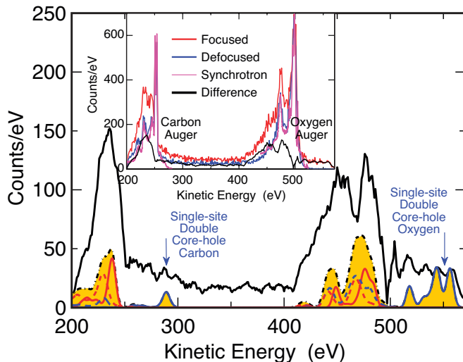
FIG. 11 (Color) Measured Auger spectra and their comparison to calculated double core-hole Auger spectra. Inset: The data are taken with different intensities and for reference at a synchrotron radiation source. Main panel: The difference of the two FEL X-ray intensities (black line) shows spectral intensity similar to the calculated spectra (yellow). Adapted from Berrah et al. , 2011.
