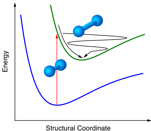
FIG. 31 (Color) A schematic of a dynamic structural change upon chemical transition. A model biatomic molecule is optically excited from the ground state to an electronic state with a different energy minimum from the ground state with respect to a structural degree of freedom.
