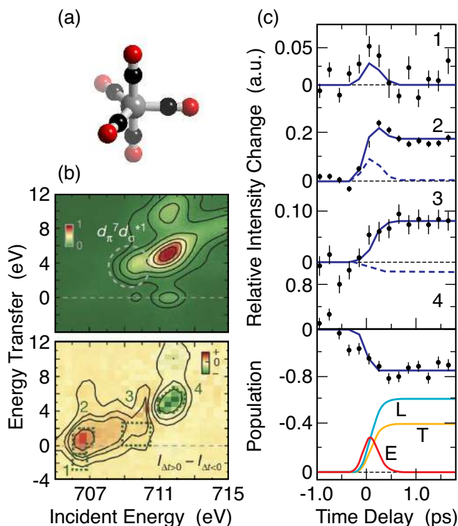
FIG. 34 (Color) Time-resolved studies of the photolysis of \text{Fe}(\text{CO})_5 . (a): Chemical structure of \text{Fe}(\text{CO})_5 ; (b): Ground state and difference RIXS map between the integrated measurements after 266 nm excitation of \text{Fe}(\text{CO})_5 solution ethanol and the ground state map. The transient intensities in the regions labelled in 1–4 (black dot symbols in (c)) have been modeled using a kinetic model using different potential electronic transition states (solid blue lines in (c)). The result of the global fit is shown in the bottom panel of (c). The compatible model includes an excited (E), triplet (T) and ethanol ligated (L) \text{Fe}(\text{CO})_4 fragment population. Simulated signals excluding a triplet and ligated population are indicated by dashed lines in panels 2 and 3. Adapted from Wernet et al. , 2015.
