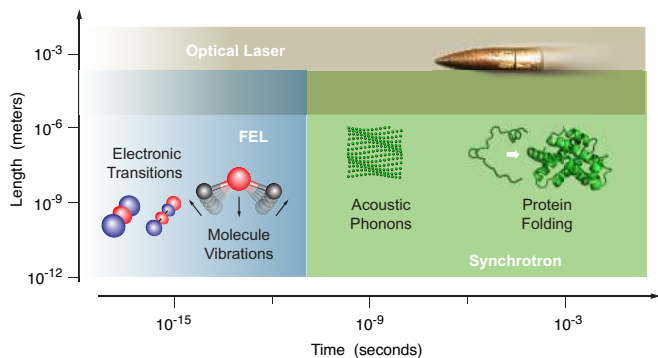
FIG. 7 (Color) Schematics of typical timescales and length scales of physical, chemical, and biological processes. Shaded regions indicate the timescales and length scales accessed by different light sources.
