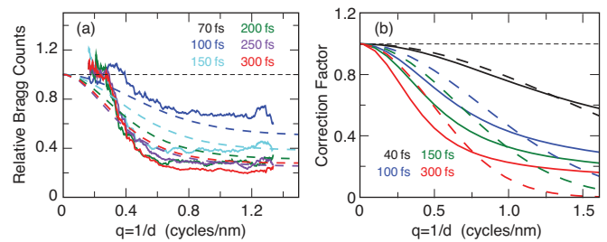
FIG. 42 (Color) Bragg termination under X-ray FEL illumination. (a) Integrated powder patterns showing the falloff of the measured Bragg intensity as a function of pulse duration for photosystem I crystals at a photon energy of 2 keV. The integrated intensity is shown relative to the shortest pulse duration (solid lines), along the simulated ratios from damage modeling (dashed lines). (b) Comparison of the simulated damage-driven disorder (solid line) with the best fit Debye-Waller factor. Reasonable agreement between the two indicates that damage can be corrected to some extent through the use of a standard resolution-dependent correction factor to the intensities. Adapted from Barty et al. , 2012.
