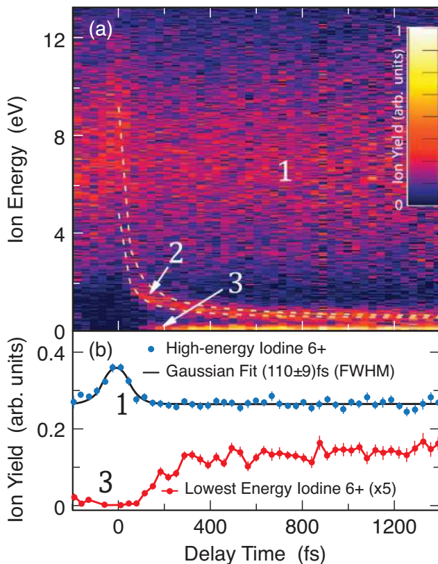
FIG. 13 (Color) Time-resolved fragmentation of CH_3I . Top panel: Map of the delay-dependent kinetic-energy distribution of I^{6+} ions following near-infrared dissociation and X-ray ionization of iodomethane. Channel 1 stems from X-ray induced dissociation of the bound molecules, channel 2 from Coulomb explosion of charged fragments, and channel 3 from X-ray ionization of the CH_3 + I^+ dissociative channel. Bottom panel: Delay-dependent yields of channel 1 and 3. Channel 3 appears only when charge transfer processes between the iodine and methyl fragments are effectively suppressed in the dissociating molecule. Adapted from Erk et al. , 2014.
