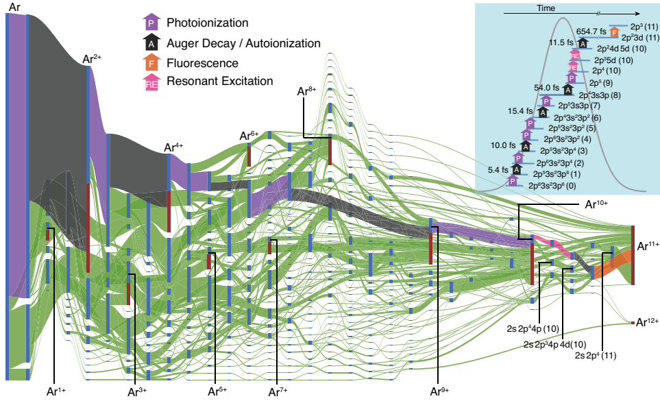
FIG. 10 (Color) Sankey diagram illustrating the transition probabilities of argon atoms illuminated with intense X-ray pulses at 480 eV. Vertical bars present possible electronic configurations, and the width of each branch indicates the transition probability. The most prominent ionization pathway to reach the highest observed charge state \text{Ar}^{11+} from the Ar ground state is highlighted in colors other than green. The inset shows the electronic configurations involved in the exemplary pathway. From Ho et al. , 2014.
