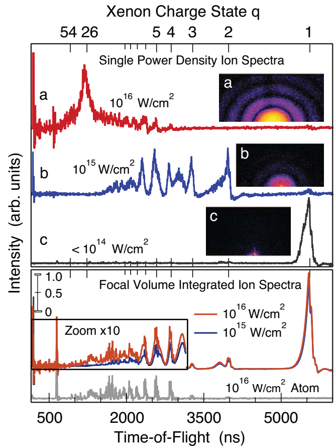
FIG. 19 (Color) Single-shot ion time-of-flight spectra of clusters irradiated with intense X-ray pulses, taken in coincidence with their diffraction image. In the three representative shots the clusters were located in the center (a) or outer wings (c) of the focus or in between (b). The ionization dynamics depend strongly on the exposure intensity. The focal volume averaged data (bottom) is dominated by the low-intensity signal in the outer wings of the focus. Adapted from Gorkhover et al. , 2012.
