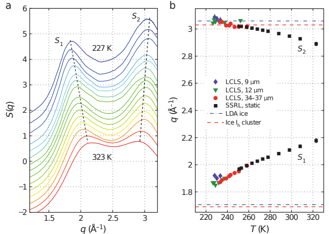
FIG. 36 (Color) Diffuse scattering profiles of metastable water, measured at different temperatures, are shown in (a). The nine lowest temperature curves were measured using ultrafast pulses from LCLS before nucleation of ice. The increasing separation of the two peaks labelled S_1 and S_2 is shown in panel (b), which approaches order peaks of low-density amorphous ice (LDA, dashdot blue lines) as well as hexagonal ice (Ice I_h , red lines). From Sellberg et al. (2014).
