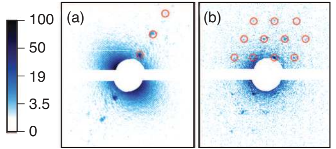
FIG. 20 (Color) Single-shot diffraction images from superfluid helium droplets doped with xenon atoms. The xenon atoms gather at the quantum vortices in the superfluid droplets, giving rise to Bragg peaks. The data suggest that the quantum vortices organize in a regular lattice with high densities. From Gomez et al. , 2014.
