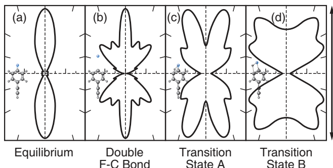
FIG. 12 Calculated fluorine 1s photoelectron angular distributions with 45 eV kinetic energy for pFAB molecule in a) the equilibrium geometry, b) with doubled F-C bond length, and in c) and d) two proposed transition states. The molecules are one-dimensionally aligned and the X-ray polarization is along the arrow. The distributions show a profound sensitivity to the local chemical environment. Adapted from Boll et al. , 2013.
