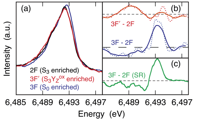
FIG. 40 (Color) K_\beta X-ray emission in photosystem II (PSII). (a) X-ray emission spectra collected on PSII solution for the doubly illuminated state (2F in black), triply illuminated state after 250 \mu\text{sec} delay (3F' in red) and triply illuminated state after 0.5 sec delay (3F in blue). (b) Difference between the LCLS-collected 3F and 2F spectra. (c) Difference between the 3F (LCLS) and 2F spectra collected at a synchrotron source at 15 K. The similarities between the LCLS and synchrotron results indicate that a similar electronic state of the manganese cluster is being probed in both cases. Adapted from Kern et al. , 2014.
