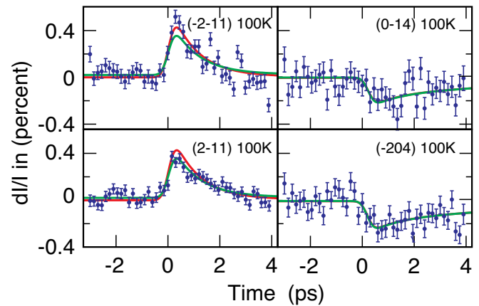
FIG. 21 (Color) Nonlinear lattice dynamics. Time-dependent Bragg reflections for four peaks in YBCO. The displacive distortion of the lattice shows a decrease in two peaks while the intensity increases in the other two. The data are for the X-ray diffraction pump-probe experiment, while the fitted curves are for the DFT with local density approximation (LDA) theory. The green shows calculations of all 11 A_g phonon modes, while the red shows the most important four: Those that couple most strongly to the optically driven, B_{1u} mode. From Mankowsky et al. , 2014.
