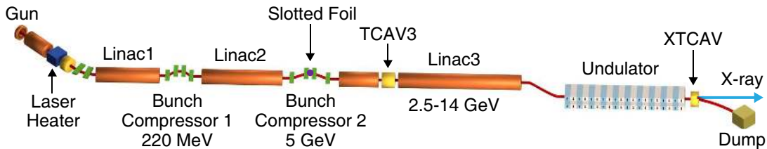
FIG. 2 (Color) Linac Coherent Light Source accelerator layout from the electron gun to the beam dump, including laser heater, two bunch compressors, three linac sections and a 132-m-long undulator. Also included are the slotted foil in the middle of Bunch Compressor 2 for X-ray pulse length control and two transverse deflecting cavities (TCAV3 and XTCAV) for pulse length measurements.
