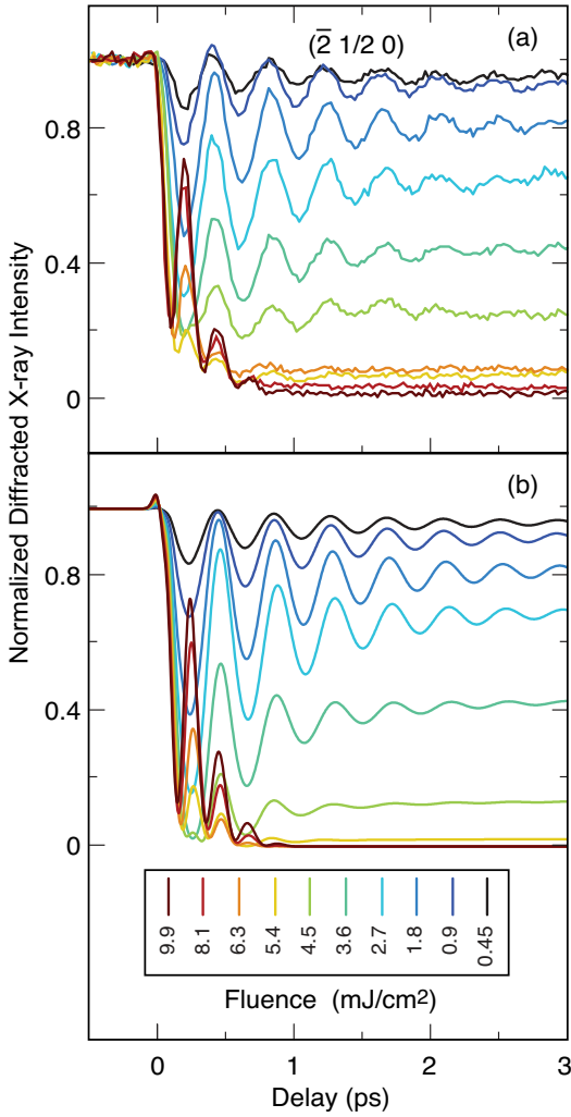
FIG. 23 (Color) The X-ray diffraction peak shown as an intensity as a function of time, describing the dynamics of the atomic structure of a \text{Pr}_{0.5}\text{Ca}_{0.5}\text{MnO}_3 manganite single crystal. The bottom panels is a simulation using a simple model based on Landau theory for a second-order phase transition. These are both shown as a function of fluence, the analog of the order parameter, used for the theoretical model. From Beaud et al. , 2014.
