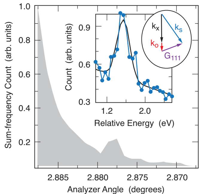
FIG. 16 (Color) X-ray and optical wave mixing signal. The additional peak at 2.878° on the sloping background of the main peak stems from sum frequency generation of the X-ray and optical pulse. The inset shows the spectral analysis of this peak, confirming that the energy of these photons equaled the sum of the incoming X-ray and optical photon frequencies. Adapted from Glover et al. , 2012.
