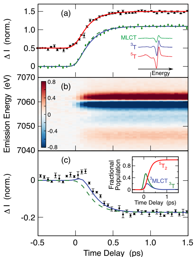
FIG. 33 (Color) Spectroscopic pump-probe results from the photoexcited spin transition of [\text{Fe}^{\text{II}}(\text{bpy})_3]^{2+} in solution. The increased iron-to-ligand distance is tracked by the XANES trace at 7125 eV ((a), black symbols, vertically offset by 0.5). The structural HS rise time has been fitted by an exponential rise of 162 \pm 6 fs (red) (Lemke et al. , 2013). (b): Time-dependent K\beta emission difference spectra. The transient traces at 7061 eV and 7054 eV have been extracted ((a)-green diamond symbols and (c)-black symbols, respectively). The data have been overlaid with results from global fits, including (blue lines) and excluding (green dashed lines) population of an intermediate {}^3\text{T} triplet ligand field state. Adapted from Zhang et al. , 2014.
