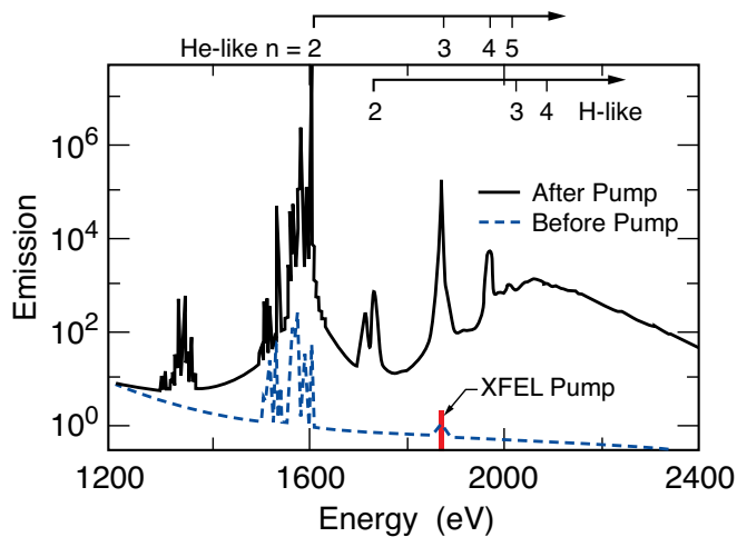
FIG. 28 (Color) The logarithm of the calculated emission spectrum from the Al plasma (blue dashed curve) and calculated emission spectrum at 100 fs after the simulated X-ray FEL pumps the He-like n=1 to n=3 transition (black solid curve). The major predicted effect of the intense X-ray pump is to cause photoionization. Adapted from Chung and Lee, 2009.
