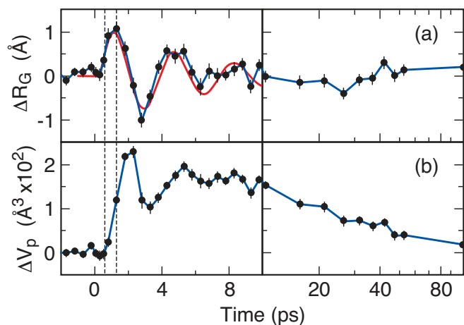
FIG. 41 (Color) Time-resolved structural changes in CO:myoglobin. (a) Damped oscillatory behavior of the radius of gyration ( \Delta R_G ) showing a 1 Å increase in 1 picosecond (ps) measured in carbonmonoxy-myoglobin (MbCO) after laser excitation. (b) Time evolution of the volume ( \Delta V_p ) of the molecule after laser excitation showing a delayed response of the volume compared to the radius of gyration. This delayed response indicates an ultrafast redistribution of the mass towards the outside solvent from the active site, verifying the existence of the protein quake. Adapted from Levantino et al. , 2015b.
