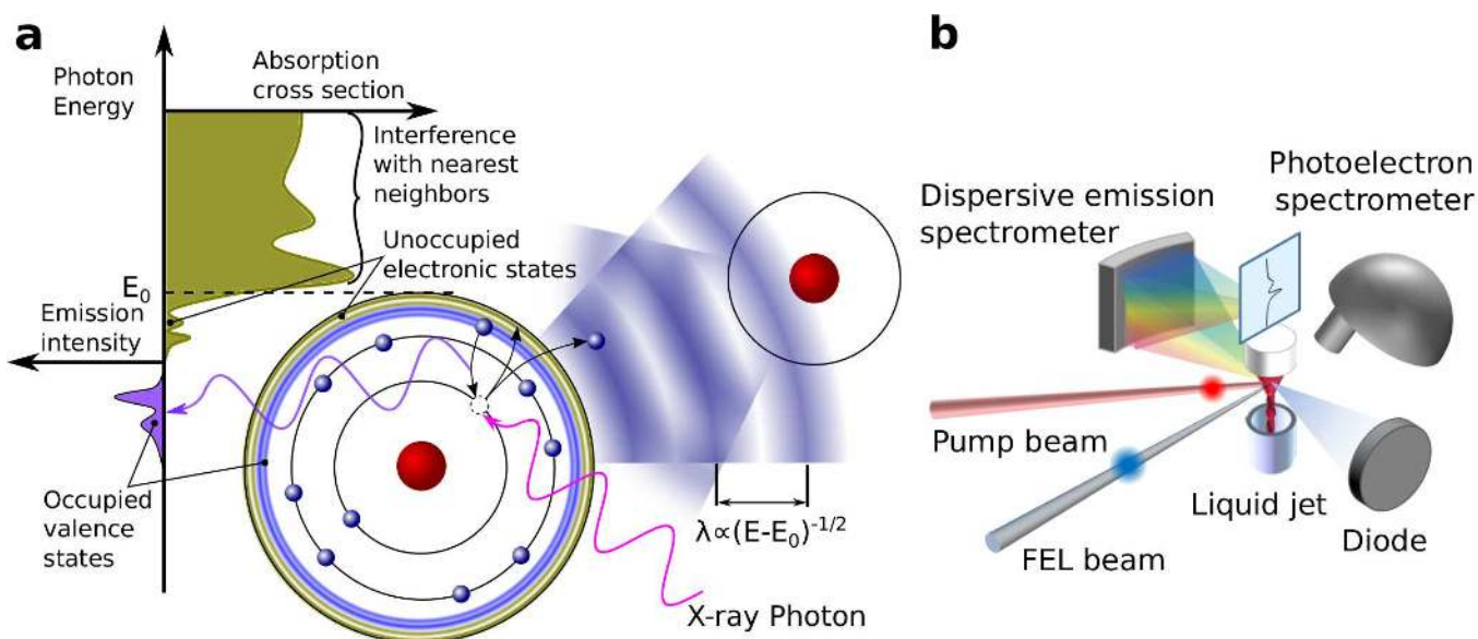
FIG. 32 (Color) A schematic representation of X-ray spectroscopy methods is shown in (a). The absorption cross section near an absorption edge of an inner-shell electron is sensitive to unoccupied electronic states just below the ionization energy E_0 and to the local structure around the excited atom. The generated hole can be occupied by a valence electron ( e.g. from a highest occupied molecular orbital state, HOMO), thereby emitting X-rays that represent electronic configurations. (b) Schematic combination of experimental ultrafast X-ray spectroscopy setups. The absorption of the monochromatic incoming X-ray pulses is measured through the total fluorescence collected by an X-ray diode. Emission spectra are measured using a dispersive spectrometer. The kinetic energy of photoelectrons can be analyzed with a photoelectron spectrometer.
