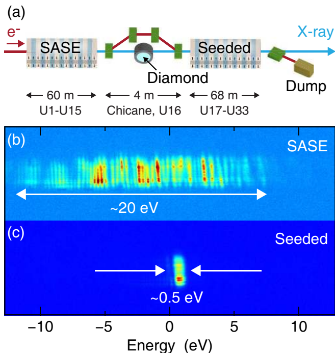
FIG. 4 (Color) Overview of hard X-ray self-seeding operation at the Linac Coherent Light Source (LCLS). Upper plot is the LCLS hard X-ray self-seeding setup at 1.5 Å (seeding diamond is not drawn to scale). Lower plots are the self-amplified spontaneous emission (SASE) and seeded spectra recorded on single shots. The seeded bandwidth (0.5 eV fwhm) is about a factor of 40 narrower than the SASE bandwidth (20 eV fwhm).
