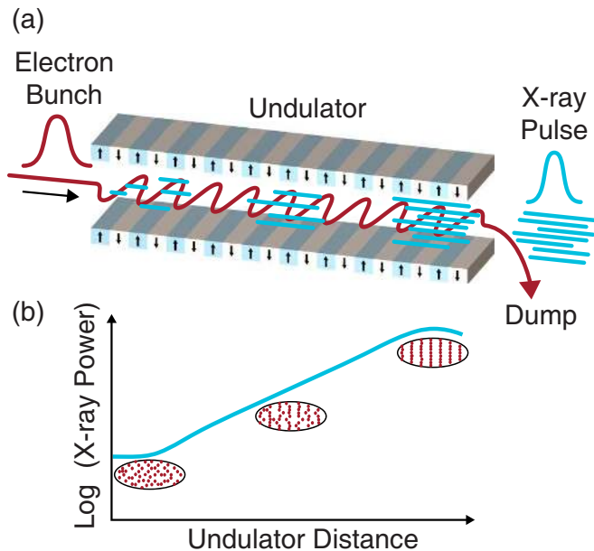
FIG. 1 (Color) Schematic of a high-gain self-amplified spontaneous emission (SASE) free-electron laser, in which both the radiation power and the electron beam microbunching grow as a function of the undulator distance until saturation.
