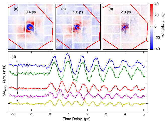
FIG. 26 Time resolved diffuse scattering measurements of Ge. (a), (b), (c) Typical frames depicting the oscillatory component of the diffuse scattering collected from the (022) Brillouin zone in Ge, after background correction, at 0.4, 1.2 and 2.8 ps. (d) A demonstration of the variation in the normalized diffuse scattering intensity as a function of time delay at select wavevectors from u = (-0.1, 0.00, -0.08) to v = (-0.33, 0.15, -0.27) in the reciprocal lattice units. From Trigo et al. , 2013.
