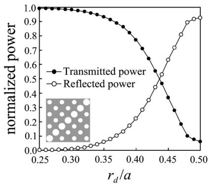
FIG. 3. The power spectra for the split beams by a line defect in a 2D square PC composed of air holes with the radius of r=0.25a as a function of r_d , the radii of defect holes. The inset represents the top view of the beam splitter structure. The calculations were done for the H -polarized mode at the frequency f=0.183c/a propagating in the \Gamma M direction with the magnetic-field parallel to the hole axes. The dielectric constant of high index background is 12.0.
