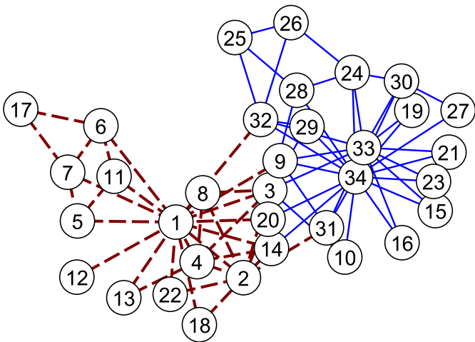
FIG. 6: (Color online) Optimal link partition into two communities of the stability R(D, 10) of the Karate club.
