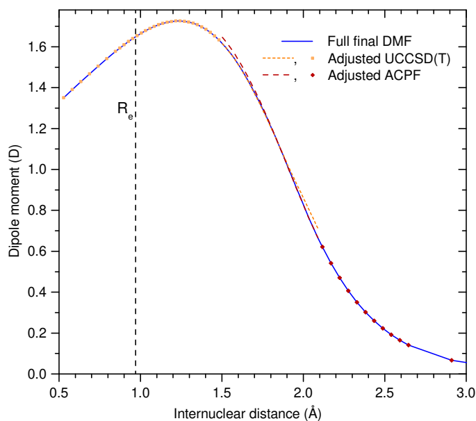
Figure 5: Mixing of the two ab initio DMFs to form a final DMF.
