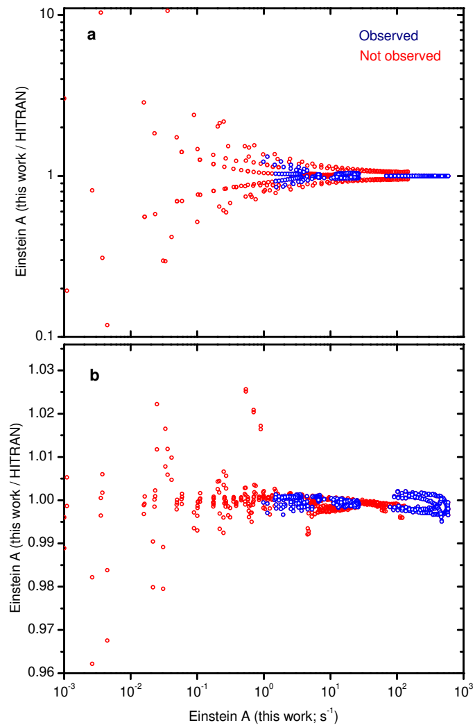
Figure 2: Ratio of Einstein A values between HITRAN and those obtained from using the methods described in this work but with the HITRAN 2012 molecular constants and DMF. a : Using the previous version of the transformation equation. b : using the final version of the transformation equation. Transitions are shown for all bands (including pure rotational) with v' up to 2, and where F' = F'' . “Observed” means that the transitions have been identified in experimental spectra, but does not refer to observed intensities.
