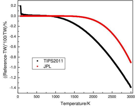
Figure 9: Relative differences between the partition sums calculated in this work, and those calculated using TIPS2011 and through direct summation of the energy levels given in the JPL database. TW stands for "this work".
