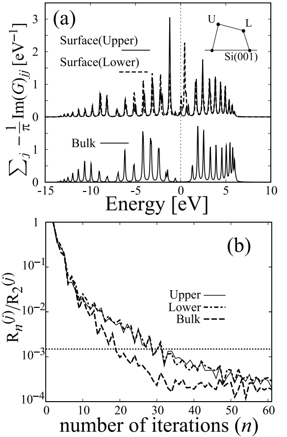
FIG. 3: Result of a slab for Si(001) surface with asymmetric surface dimers; (a) Local density of states ( \sum_j -1/\pi \text{Im}G_{jj} ) for surface and bulk atoms, calculated with the KS dimension of n = 30 . The surface atoms are classified into the upper and lower atoms of the asymmetric dimer, illustrated in the inset. The ‘bulk’ atom is an atom on deeper layers of the present slab system. (b) Decay behavior of a-RN for the atoms that appear in (a). The horizontal dotted line is an eyeguide for a typical convergence criteria.
