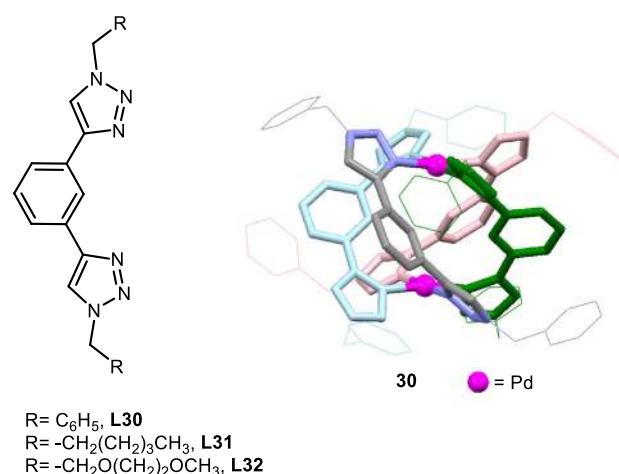
Figure 26. Ligand L30 , X-ray structure of [Pd 2 (L30) 4 ](BF 4 ) 4 , 30 showing a quadruple-stranded helicate using 1,2,3-triazole as a ligand. (Hydrogen atoms and non-coordinating anions are not shown for clarity).
