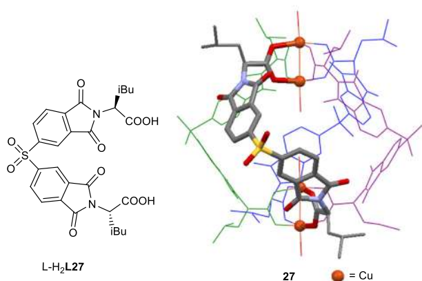
Figure 23. L-leucine-derived ligand H 2 L27 and X-ray structure of \Lambda -[Cu 4 (L-L27) 4 ], 27 showing a quadruple-stranded helicate (coordinated solvent displayed only by the donor atom for clarity, hydrogen atoms and non-coordinating anions are not shown for clarity).
