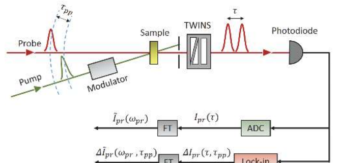
Fig. 7. Sketch of the setup used for broadband pump-probe spectroscopy and SRS.
