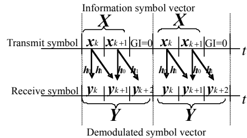
Figure 3. Illustration of zero-padding to prevent IBI at receiver on MIMO multipath channel ( L=2, N=2 ).
