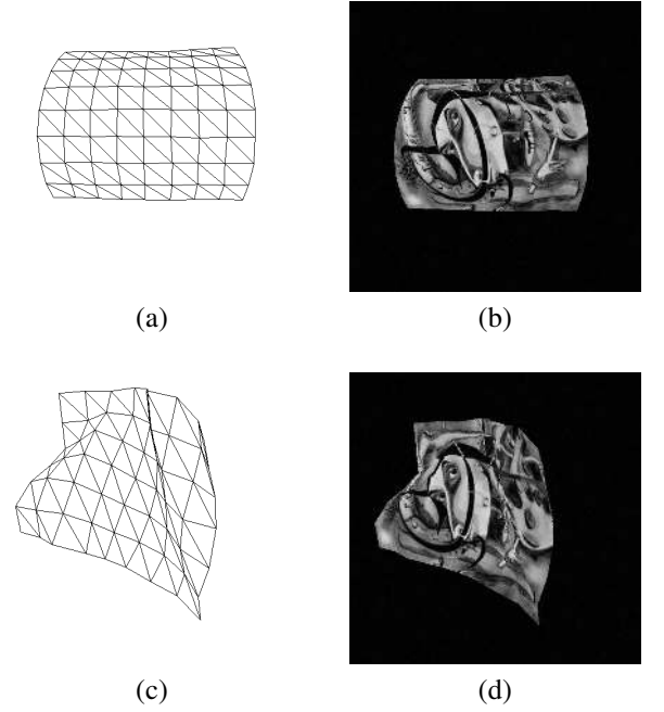
Fig. 9. Synthetic data acquired with a motion capture system. (a,b) Mesh and corresponding textured image of a smoothly deforming piece of cardboard. (c,d) Similar images for a piece of cloth with sharper folds.
