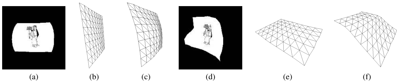
Fig. 17. Recovering the shape of poorly textured surfaces (a,d). (b,e) 3D reconstruction using equality constraints. (c,f) 3D reconstruction using inequality constraints. Since we only exploit shape information in the center of the image, the recovered surfaces are far too smooth.
