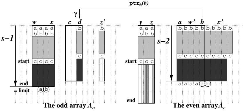
Fig. 2. Finding \gamma at stage s .
