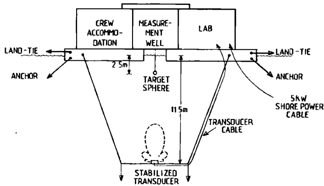
FIG. 1. Measurement configuration.
