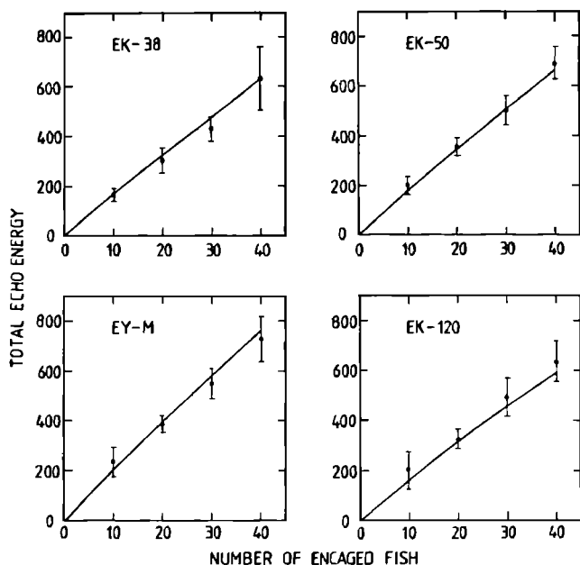
FIG. 5. Comparison of theoretical and measured values of total echo energy from the encaged herring aggregations. The echo energy has been expressed in units of square centimeters. Experimental points are indicated with confidence intervals defined at twice the estimated standard deviation. Theory is indicated by the solid line.
