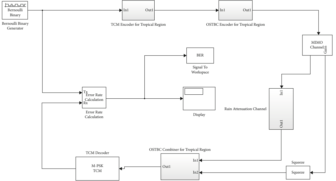
FIGURE 2: Communication link model for 5G communication in the tropical regions.
